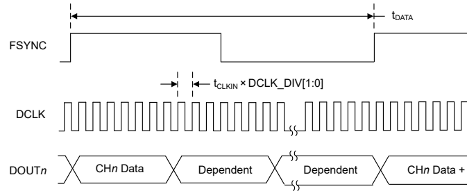
Figure 7-31. Frame-Sync Port Operation
