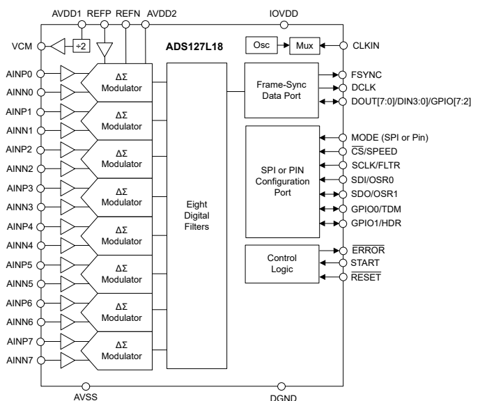
Functional Block Diagrams
