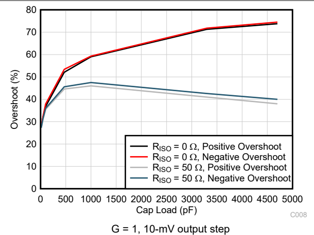
Figure 5-28. Small-Signal Overshoot vs Capacitive Load
