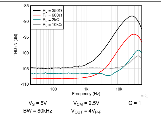
Figure 6-40. THD + N vs Frequency
