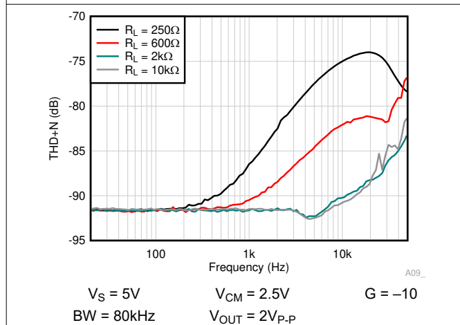
Figure 6-39. THD + N vs Frequency
