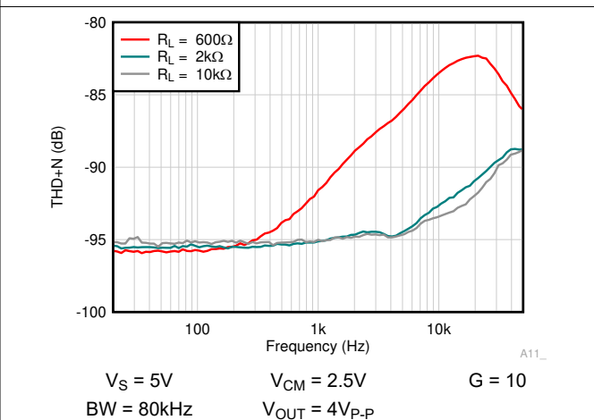
Figure 6-42. THD + N vs Frequency
