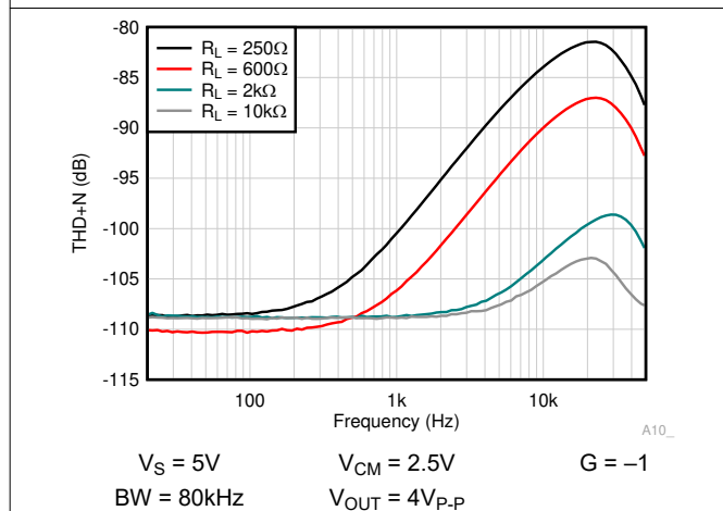
Figure 6-41. THD + N vs Frequency
