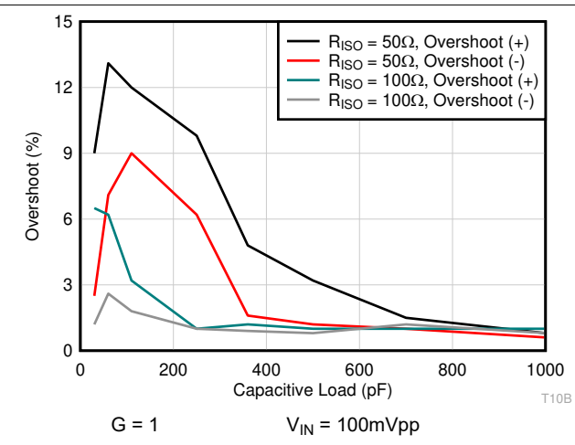
Figure 6-54. Small Signal Overshoot vs Capacitive Load
