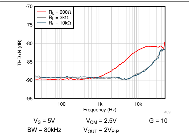
Figure 6-38. THD + N vs Frequency
