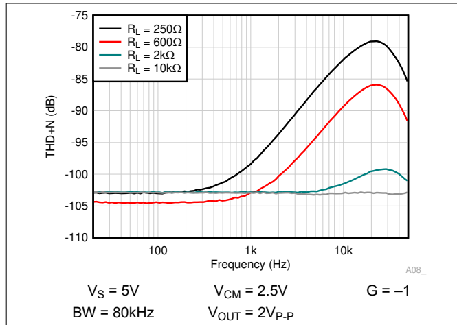
Figure 6-37. THD + N vs Frequency
