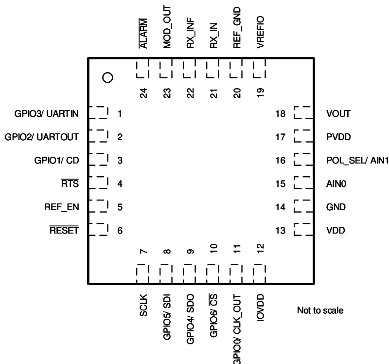
Figure 4-1. Pin Diagram
