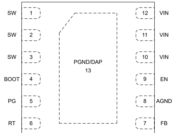
Figure 4-1. Pin Diagram
