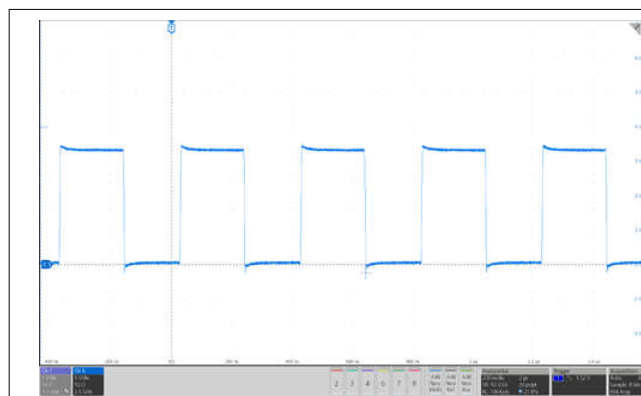
DR = 5 Mbps ISOM8710 V_{CC} = 3.3 \text{ V} C_L = 15 \text{ pF} Figure 10-2. Typical Output Waveform at I_F = 2 \text{ mA}
