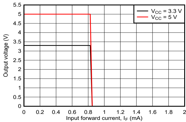
Figure 7-3. Output Voltage vs Input Forward Current
