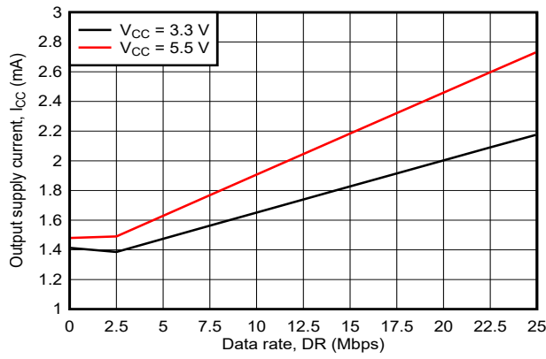
I_F = 6 \text{ mA} ISOM8710 C_L = 15 \text{ pF} Figure 7-13. Output Supply Current vs Data Rate
