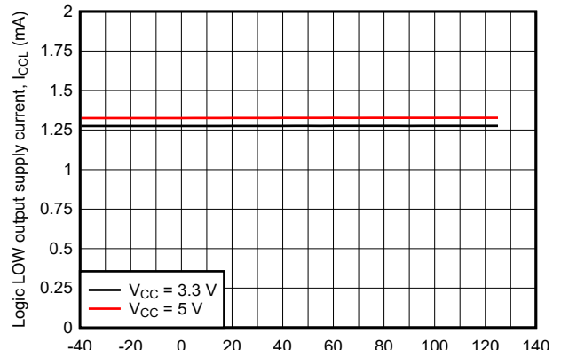
I_F = 6 \text{ mA} ISOM8711 Figure 7-16. Logic LOW Output Supply Current vs Ambient Temperature
