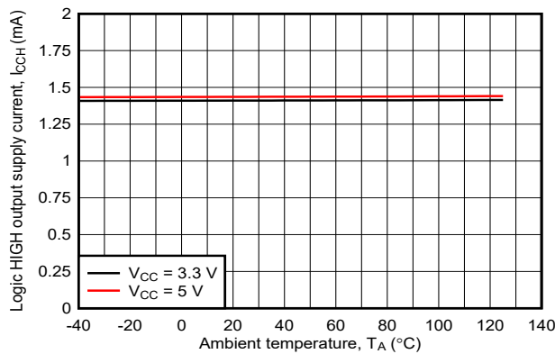
I_F = 0 \text{ mA} ISOM8710 Figure 7-17. Logic HIGH Output Supply Current vs Ambient Temperature
