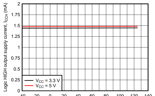
I_F = 0 \text{ mA} ISOM8711 Figure 7-18. Logic HIGH Output Supply Current vs Ambient Temperature
