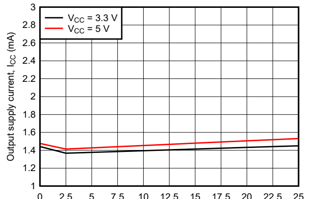
I_F = 6 \text{ mA} ISOM8711 C_L = 15 \text{ pF} Figure 7-14. Output Supply Current vs Data Rate
