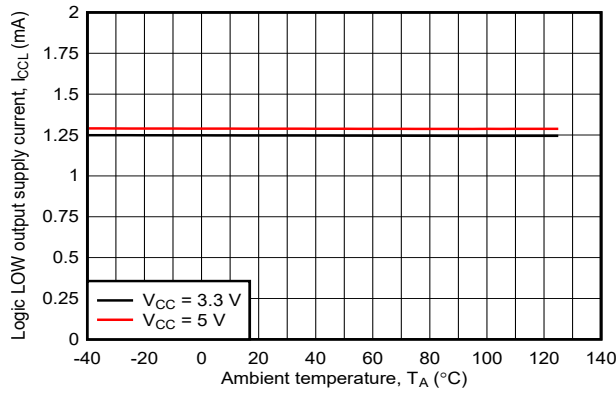
I_F = 6 \text{ mA} ISOM8710 Figure 7-15. Logic LOW Output Supply Current vs Ambient Temperature
