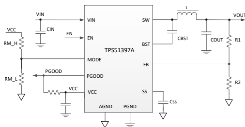
Simplified Schematic
