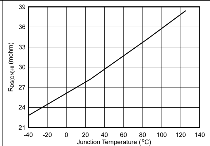
Figure 6-6. High-Side R_{DS(ON)}
