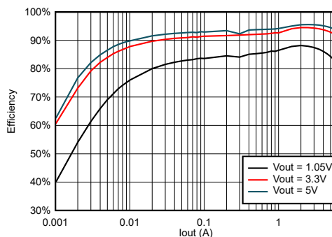
TPS566242, Efficiency at VIN = 12 V
