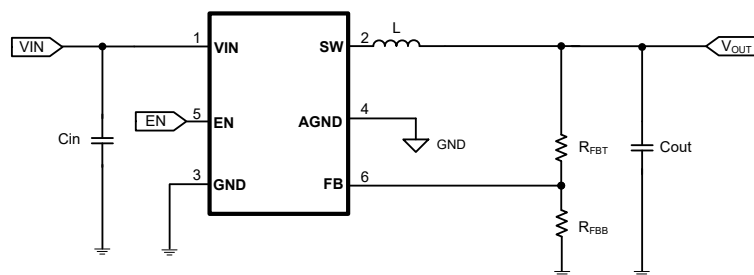
Simplified Schematic
