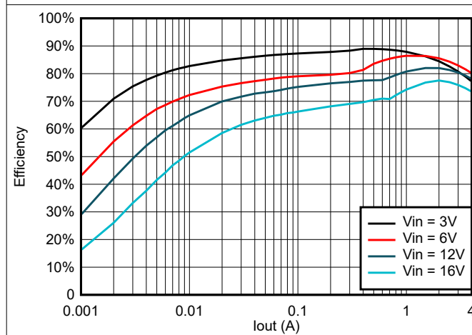
Figure 6-11. TPS564242 Efficiency at 0.6\text{ V}_{OUT} with a 0.82\text{-}\mu\text{H} Inductor
