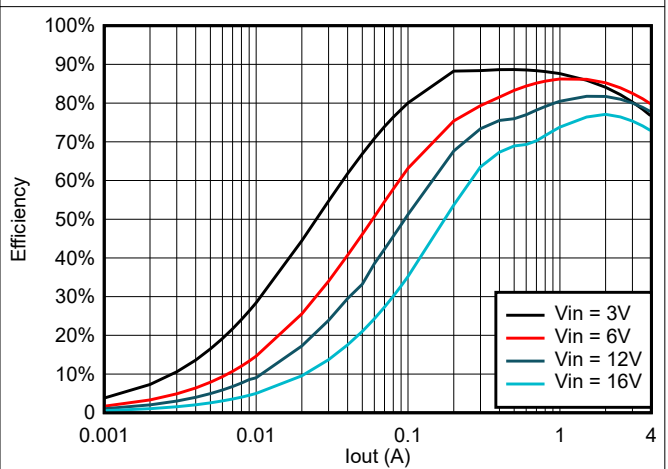
Figure 6-12. TPS564247 Efficiency at 0.6\text{ V}_{OUT} with a 0.82\text{-}\mu\text{H} Inductor
