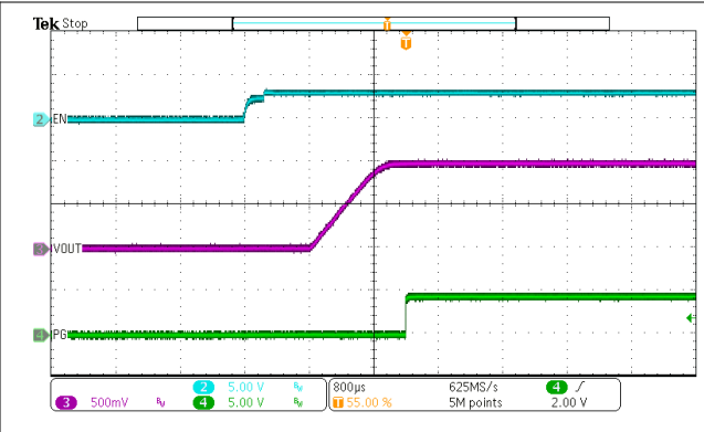
Figure 7-11. EN Start-Up – With Load
