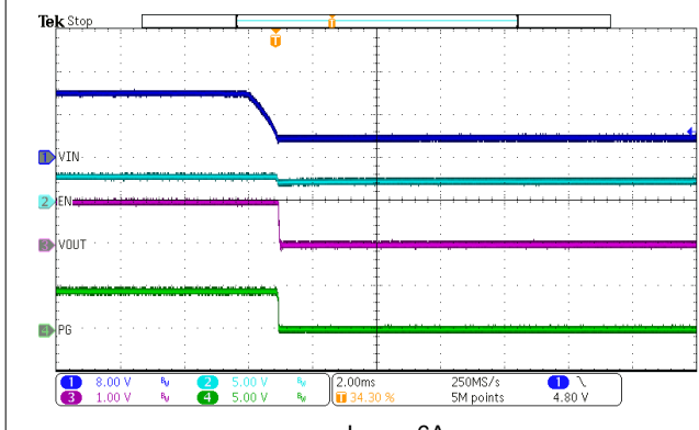
Figure 7-14. VIN Shutdown
