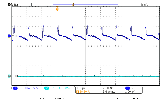
Figure 7-15. Output Ripple – No Load
