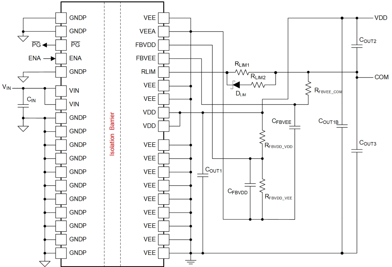
Figure 8-9. Dual output application schematic configured for V_{\text{COM\_VEE}} regulation = 2.5V
