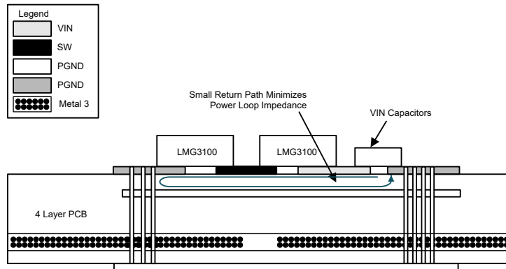
Figure 9-5. Four-Layer Board Cross Section With Return Path Directly Underneath for Power Loop
