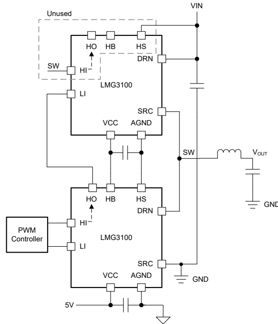
Figure 9-1. Typical Connection Diagram For a Synchronous Buck Converter
