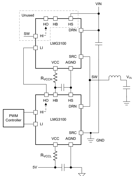
Figure 9-2. Slew Rate Control with R_{VCCL} and R_{VCCH} Resistors
