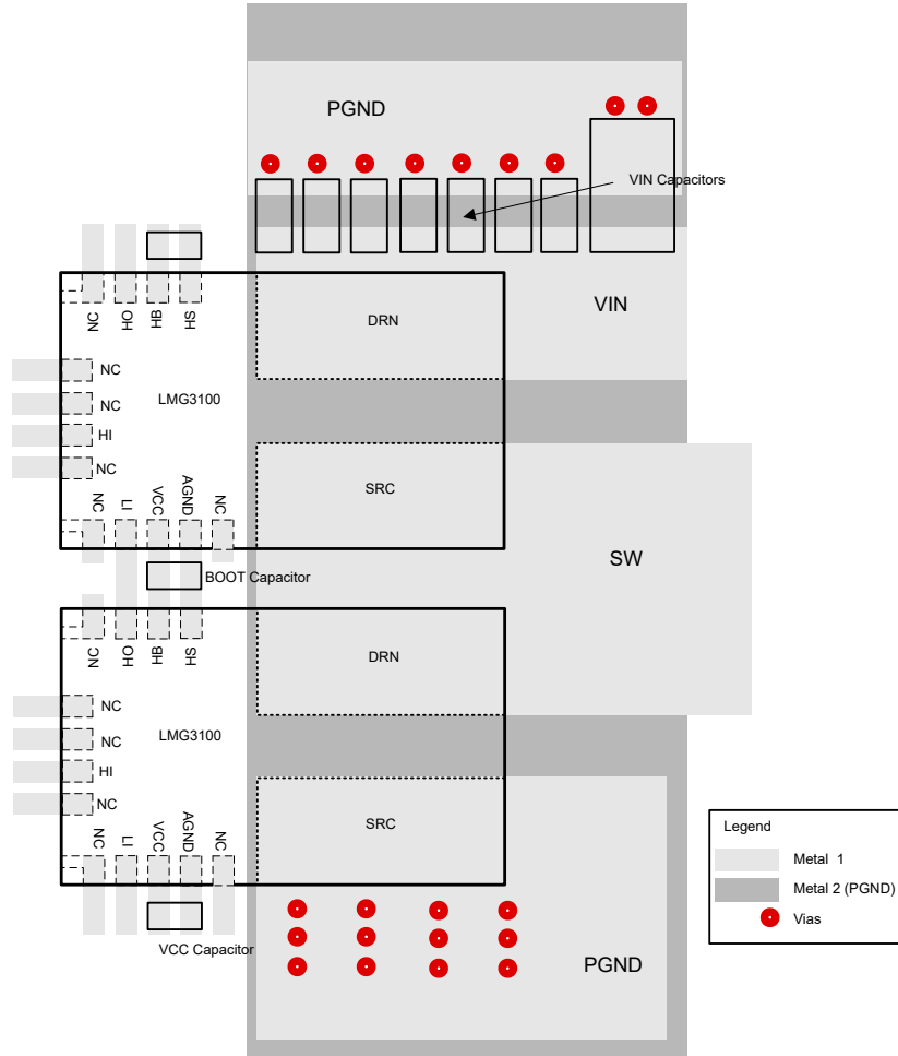
Figure 9-4. External Component Placement (Multi Layer Board)
