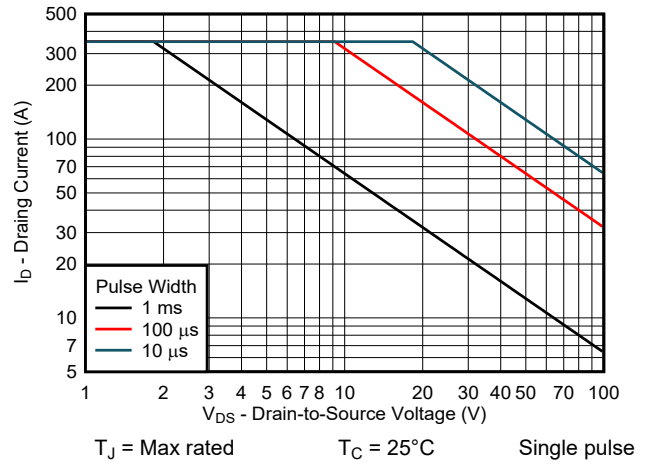
Figure 6-2. Safe Operating Area
