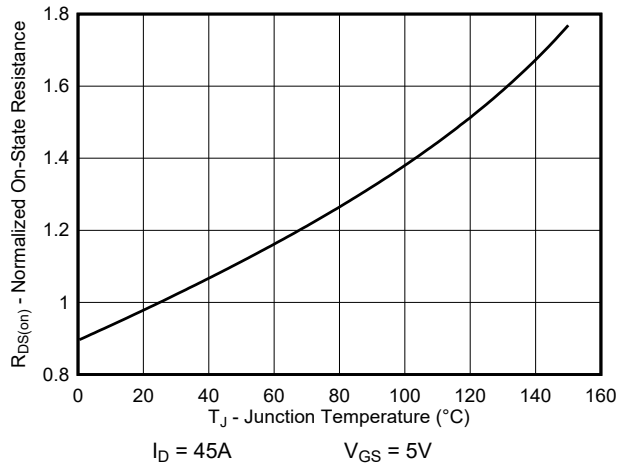
Figure 6-1. Normalized On-State Resistance vs Junction Temperature
