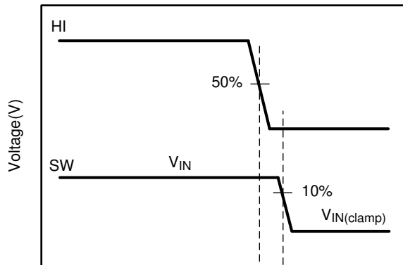
Figure 7-4. High-Side Gate Driver Turnoff
