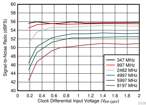
JMODE 1, FG calibration, f_S = 6400\text{ MSPS} , A_{IN} = -1\text{ dBFS}
