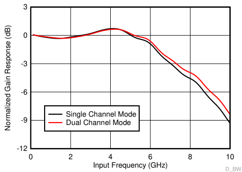
Figure 6-68. Gain Response vs Input Frequency
