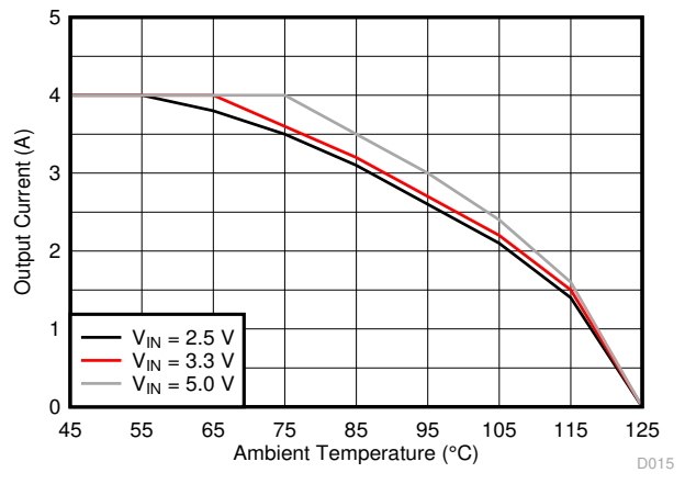
Figure 8-30. Thermal Derating
