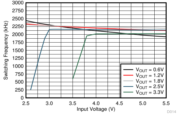
Figure 8-28. Switching Frequency
