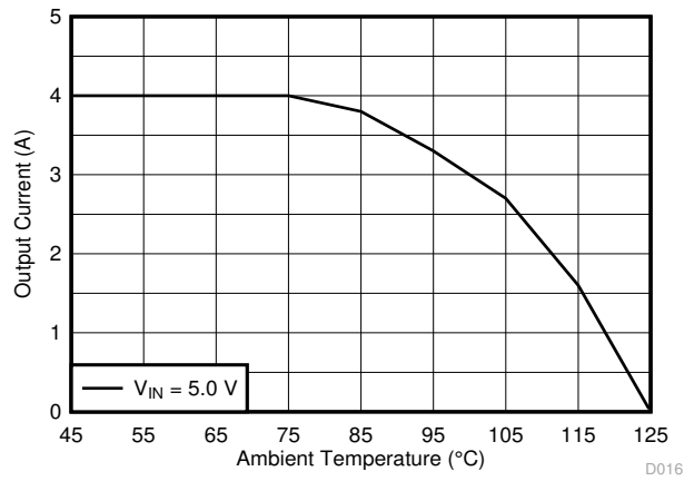
Figure 8-32. Thermal Derating
