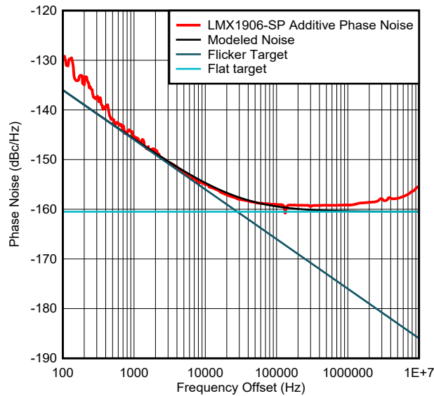
Figure 5-6. LMX1906-SP Flicker Noise
