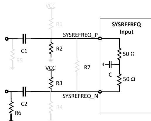
Figure 7-3. AC-Coupled, Single-Ended Input
