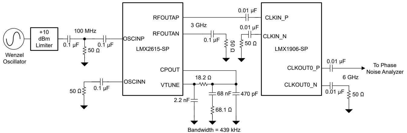
Figure 7-6. Typical Application Schematic
