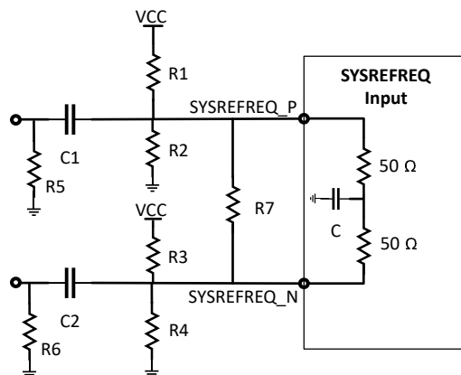
Figure 7-1. SYSREFREQ Input Circuit Recommendations
