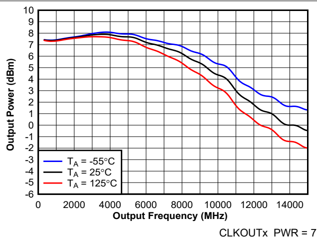
Figure 5-10. Buffer Mode Single-Ended Output Power
