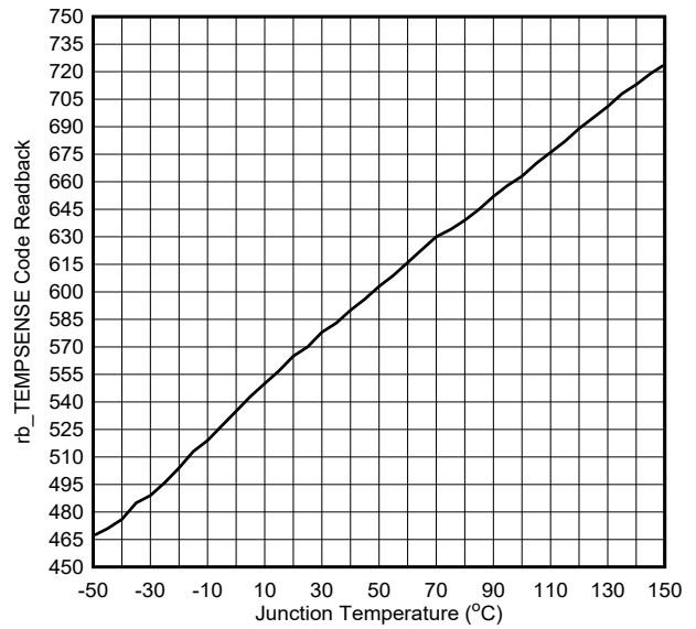
Figure 5-17. Temperature Sensor Readback
