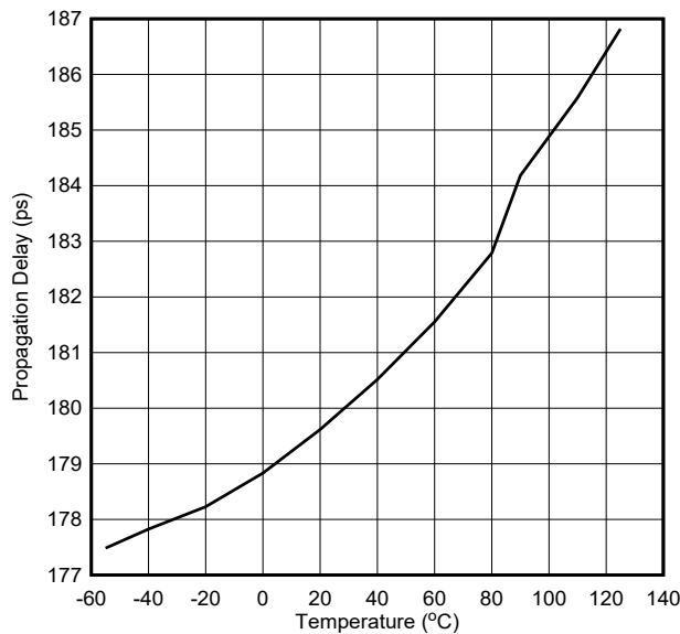
Figure 5-18. Propagation Delay
