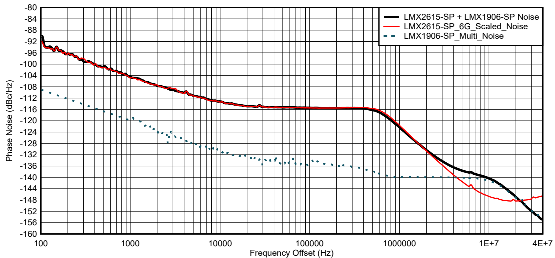
Figure 7-8. LMX1906-SP Multiplier Output
