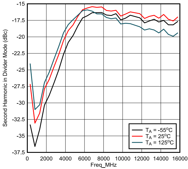
Figure 5-14. Second Harmonic on Divider Mode (Single-Ended Input)
