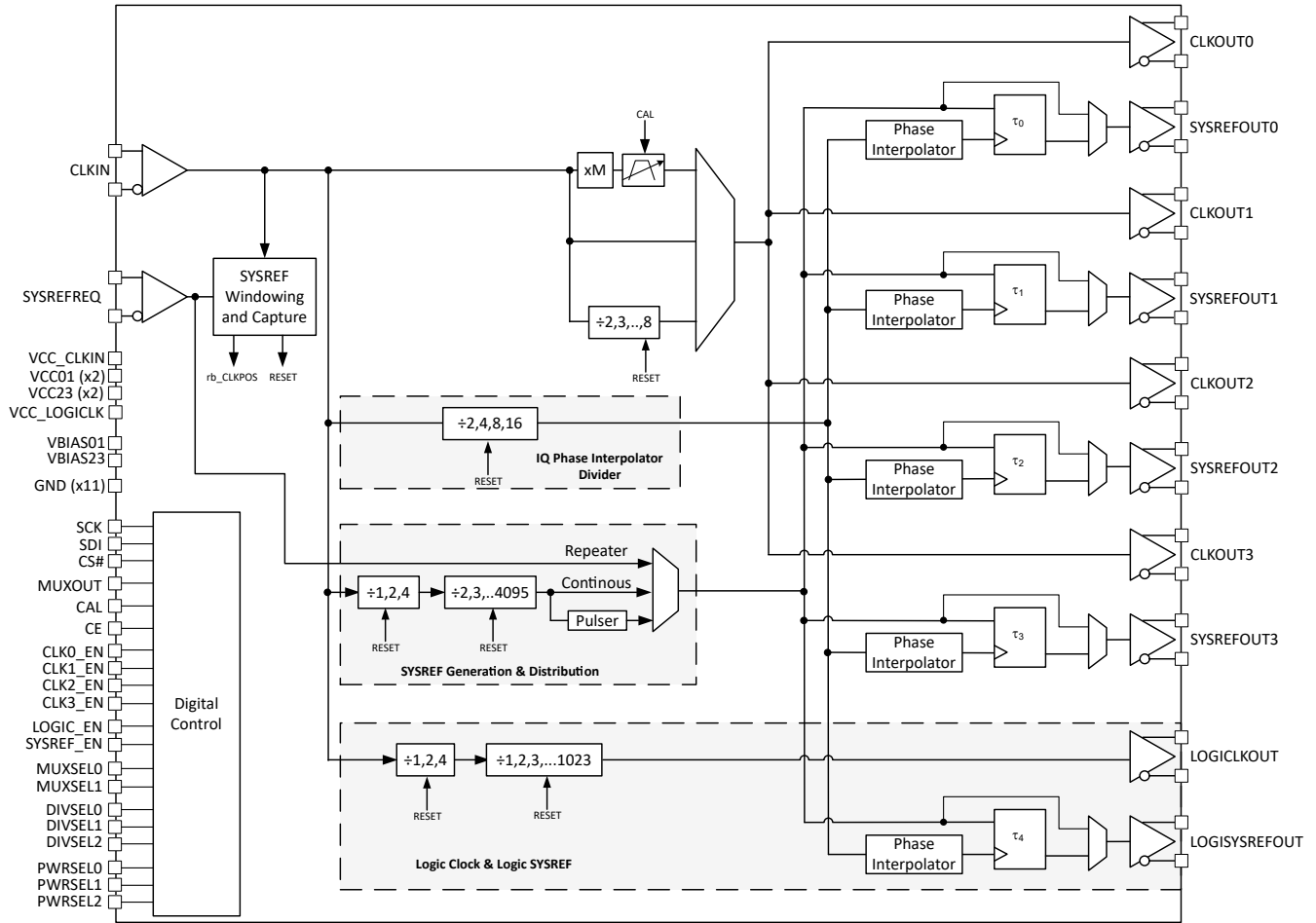
Block Diagram
