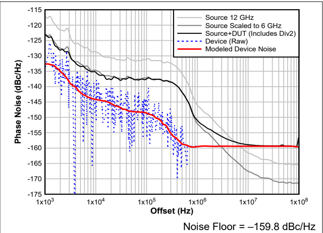
Figure 5-3. Divider Phase Noise Plot at 6 GHz Output (Divide by 2)
