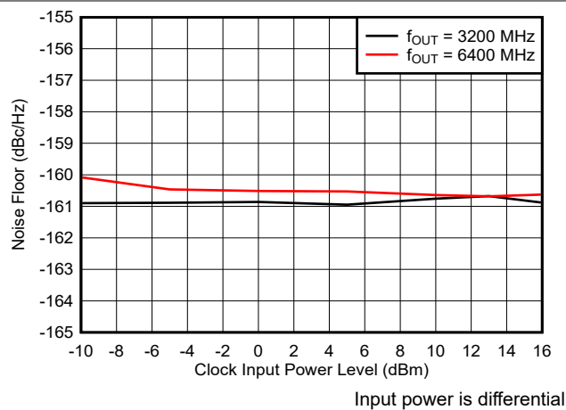
Figure 5-8. Noise Floor in Multiply x2 Mode
