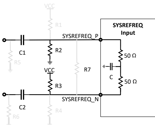
Figure 7-2. AC-Coupled Differential Input
