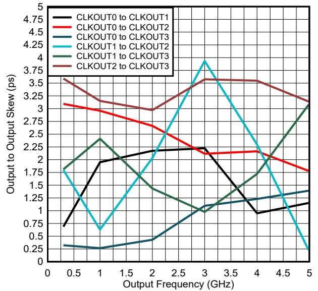
Figure 5-15. Output to Output Skew (ps)
