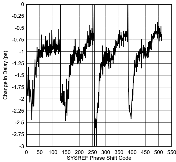
Figure 5-16. SYSREF Delta Delay vs. Code
