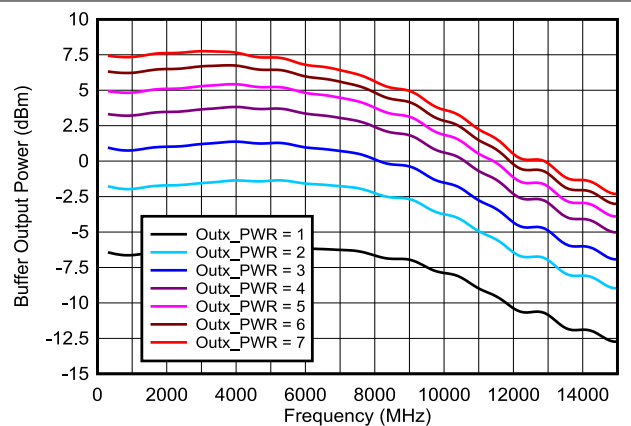
Figure 5-9. Buffer Mode Single-Ended Output Power
