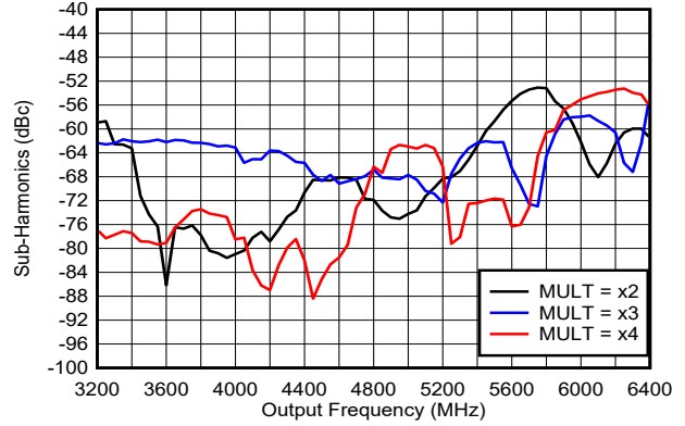
Figure 5-13. Multiplier Sub-Harmonics (Harmonic Frequency = Output Frequency / M)
