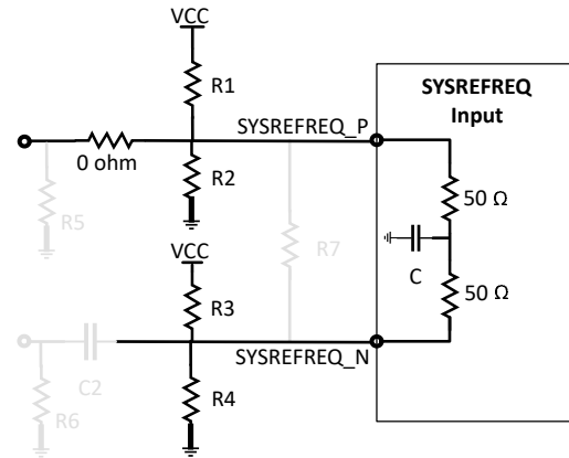
Figure 7-5. DC-Coupled, Single-Ended Input
