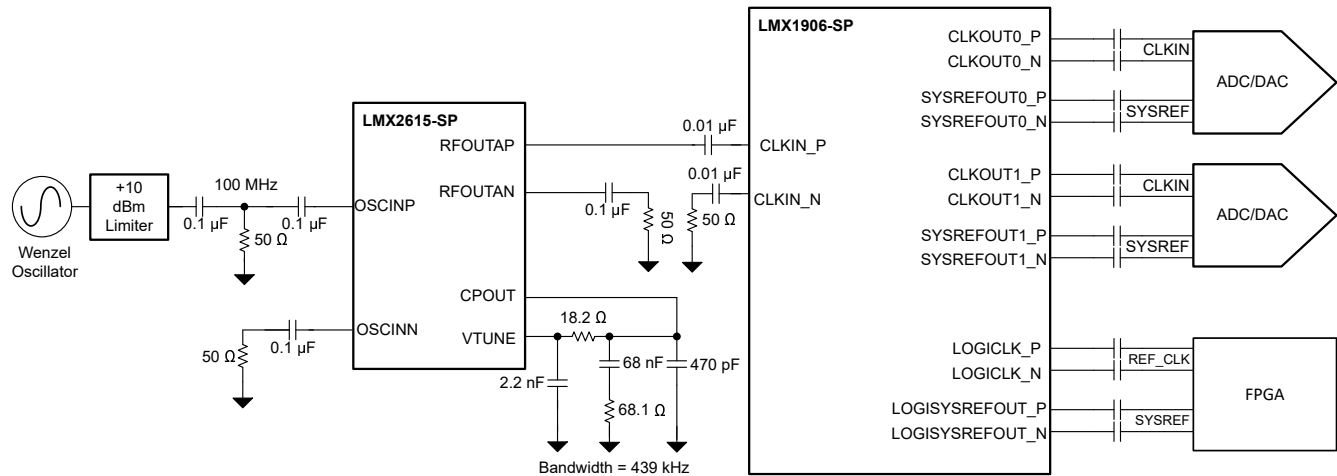
Figure 7-9. Typical JESD Clocks Block Diagram
