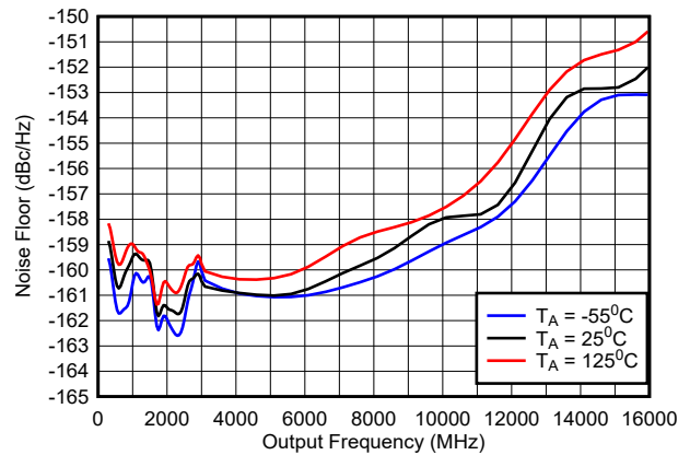
Figure 5-7. Noise Floor in Buffer Mode
