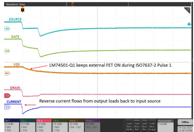
Figure 9-4. Response to ISO 7637-2 Pulse 1
