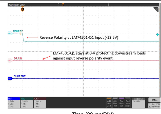
Figure 9-10. Input Reverse Polarity Hot Plug
