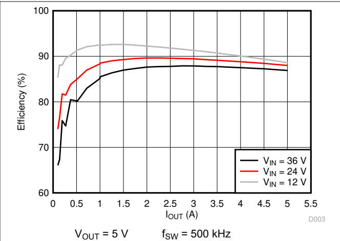
Figure 5-2. Efficiency versus Load Current
