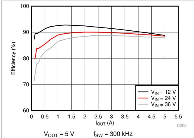
Figure 5-1. Efficiency versus Load Current
