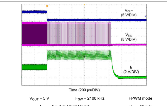
Figure 10-20. LM62440-Q1 Short Circuit Protection
