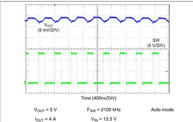
Figure 10-18. LM62440-Q1 Switching Waveform and V_{OUT} Ripple
