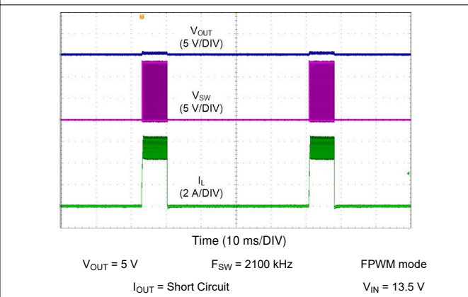
Figure 10-22. LM62440-Q1 Short Circuit Performance
