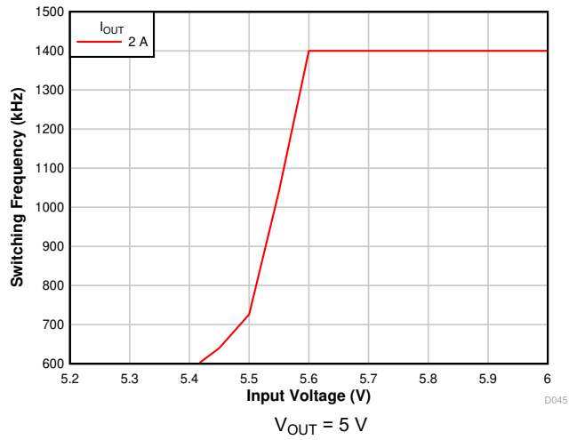
Figure 7-10. Frequency Foldback
