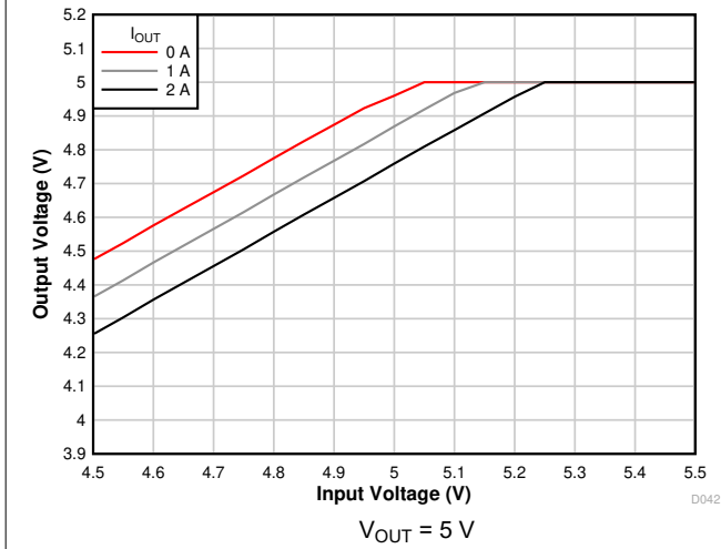
Figure 7-9. Voltage Dropout
