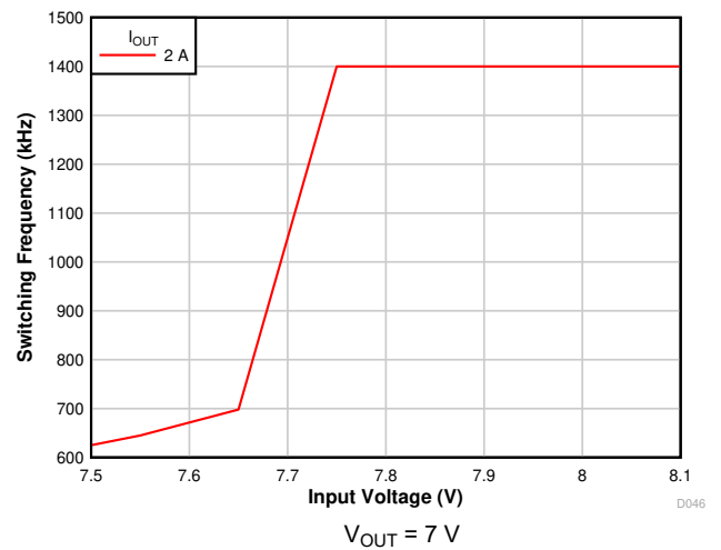
Figure 7-12. Frequency Foldback
