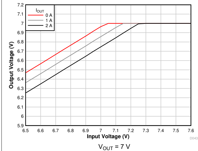
Figure 7-11. Voltage Dropout
