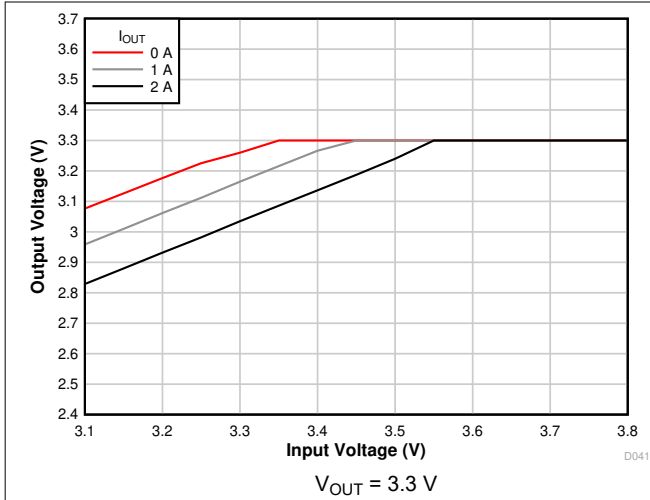
Figure 7-7. Voltage Dropout
