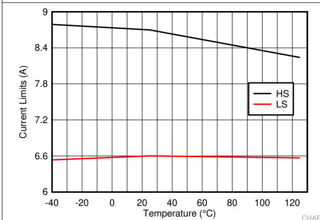
Figure 6-5. TPS7H4010-SEP High-Side and Low-Side Current Limit
