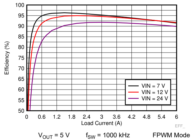
Figure 8-6. TPS7H4010-SEP Efficiency
