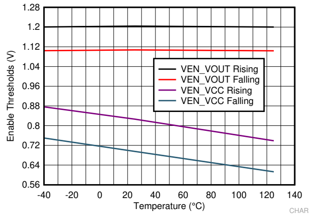
Figure 6-8. Enable Thresholds
