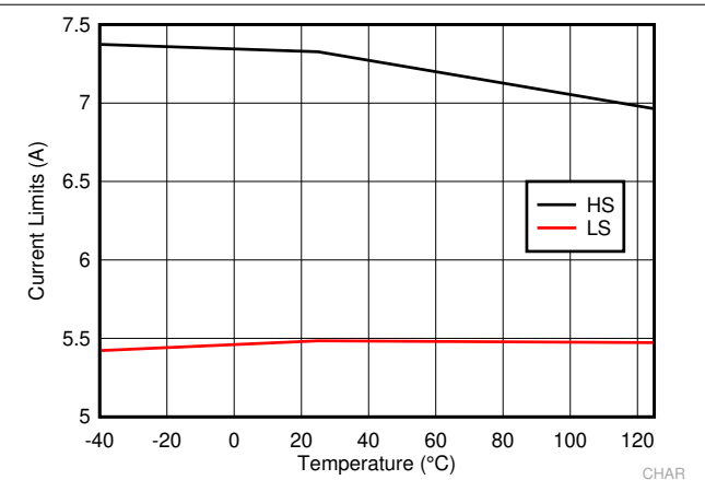
Figure 6-4. TPS7H4010-SEP High-Side and Low-Side Current Limits
