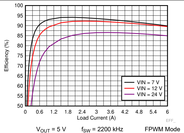
Figure 8-8. TPS7H4010-SEP Efficiency
