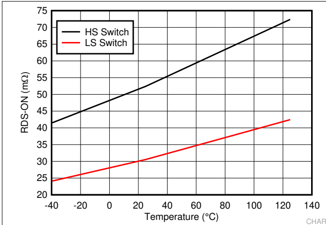
Figure 6-1. High-Side and Low-Side Switches RDS-ON
