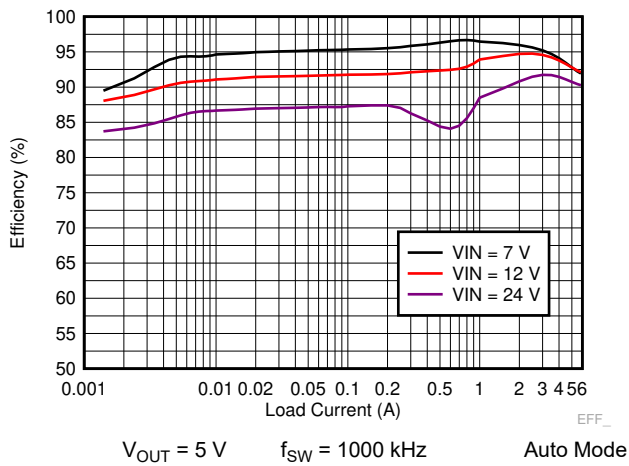
Figure 8-5. TPS7H4010-SEP Efficiency
