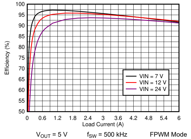
Figure 8-4. TPS7H4010-SEP Efficiency
