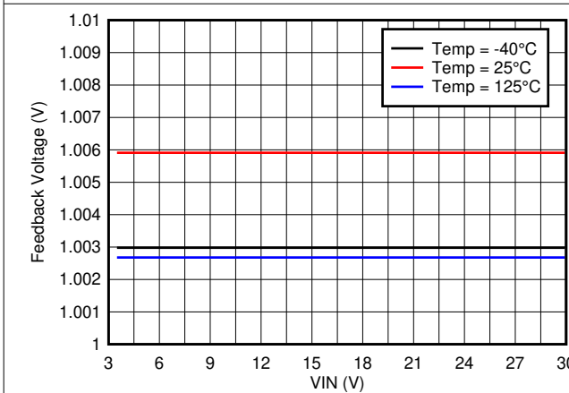
Figure 6-3. Feedback Voltage
