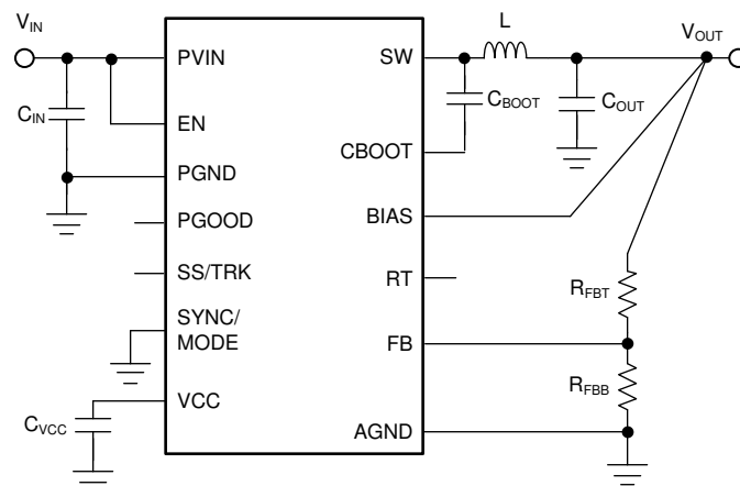
Figure 8-1. TPS7H4010-SEP Basic Schematic
