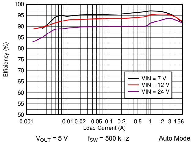
Figure 8-3. TPS7H4010-SEP Efficiency
