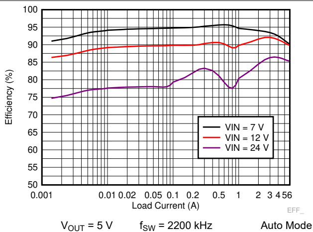
Figure 8-7. TPS7H4010-SEP Efficiency
