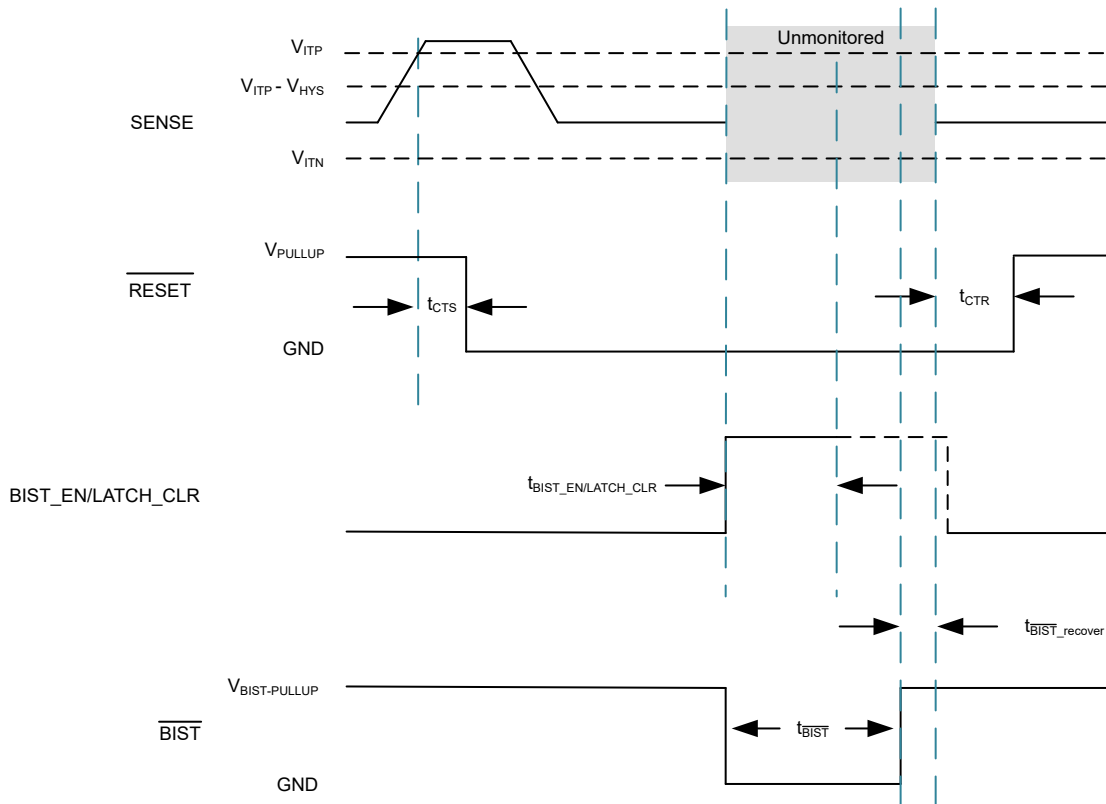
Figure 10-6. \overline{\text{RESET}} Latch & Unlatch
