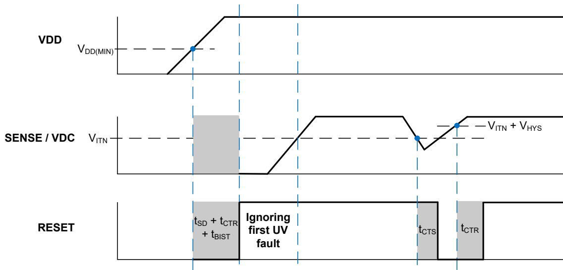
Figure 10-8. UVbypass Enabled
