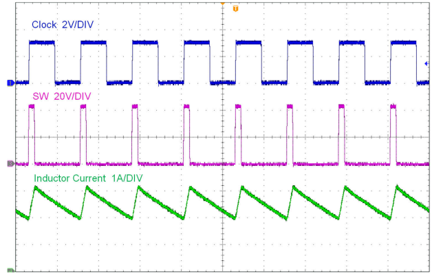
LMR38025 V_{OUT} = 5V 400kHz 2 \mu s/DIV
