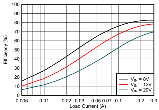
Figure 8-7. Efficiency
