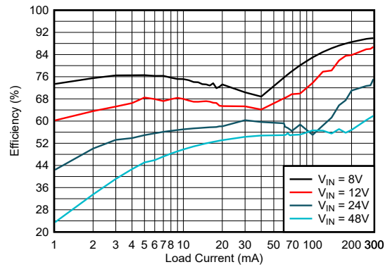
Figure 8-4. Efficiency
