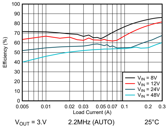
Figure 8-4. Efficiency
