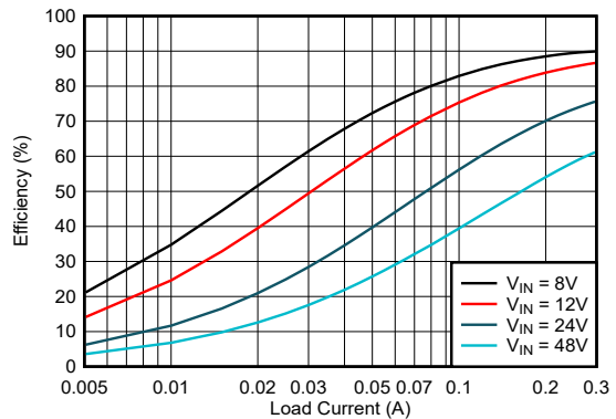
Figure 8-5. Efficiency
