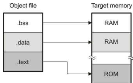
Figure 2-1. Partitioning Memory Into Logical Blocks
