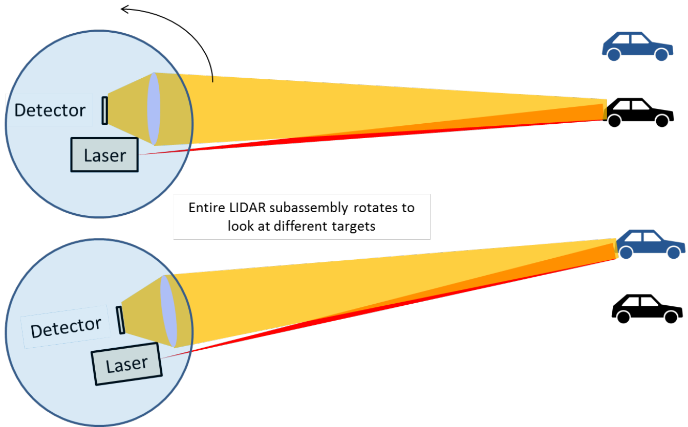
Figure 2. Mechanical LIDAR architecture
