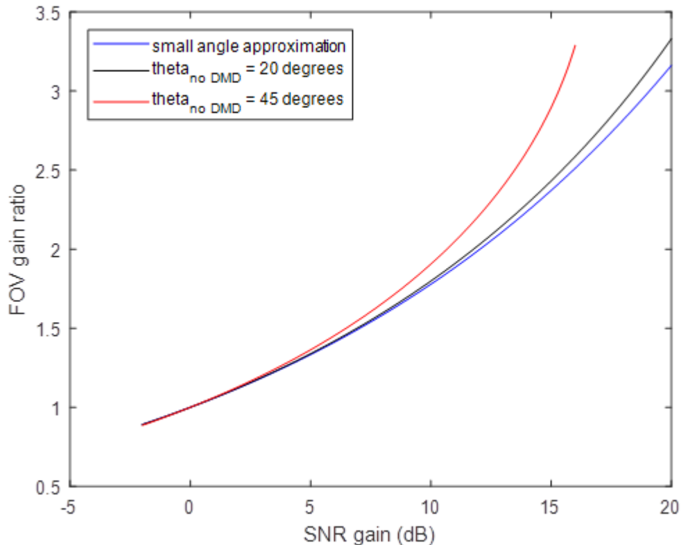
Figure 7. Small angle approximation for SNR vs FOV expansion
