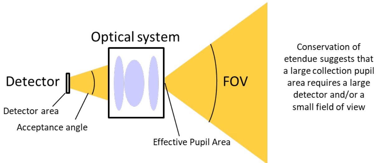
Figure 5. Relationship between detector etendue and system FOV
