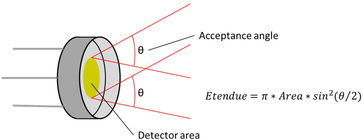
Figure 4. Etendue of a photodetector
