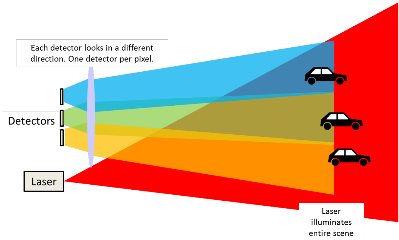
Figure 1. Flash LIDAR architecture
