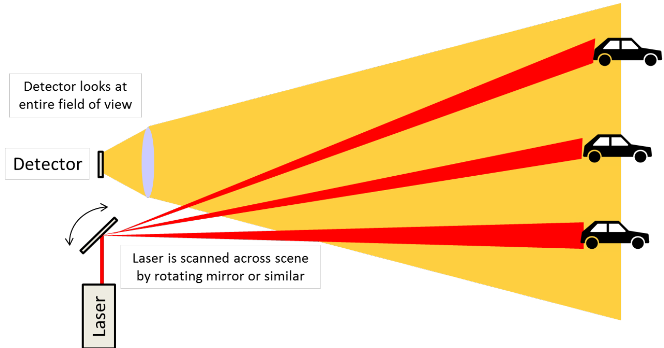
Figure 3. Scanning LIDAR architecture
