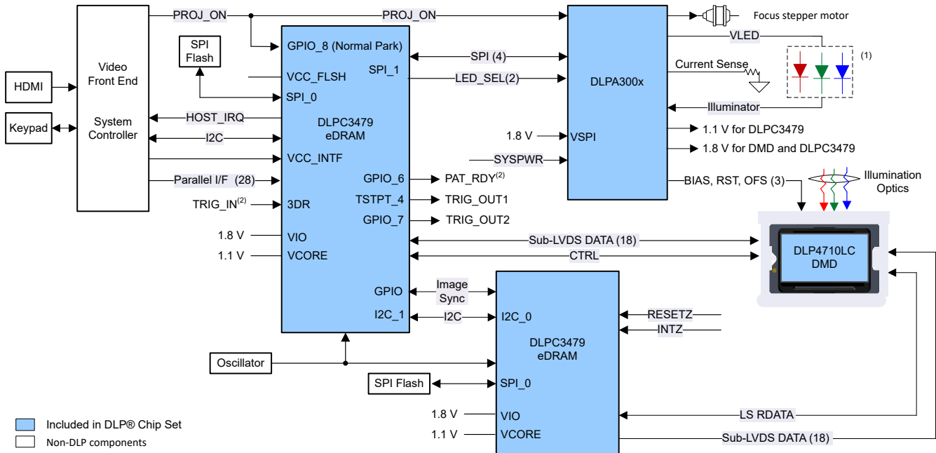
Figure 1-1. DLPC3479 System Block Diagram
