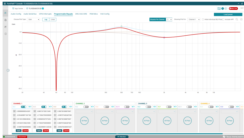
Figure 3-3. PurePath™ Console Programmable Biquad Filter Example Showing the Computed Coefficients in Normalized Floating Point Format
