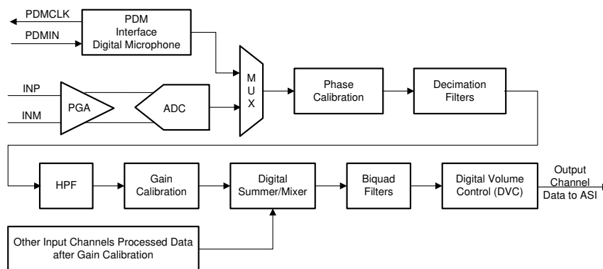
Figure 1-1. TLV320ADCx120 and PCMx120-Q1 Channel Signal Chain Processing Flow Chart
