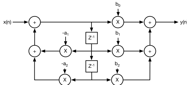
Figure 2-1. Direct Form II Biquad Filter
