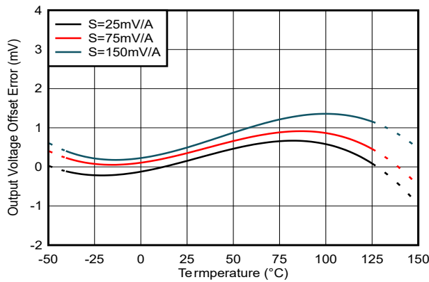
Figure 6-3. Offset Error vs Temperature: TMCS1133Bxx Device Options
