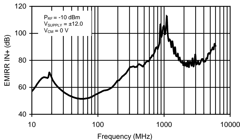
Figure 1. TLE2071 EMIRR IN+ vs Frequency
