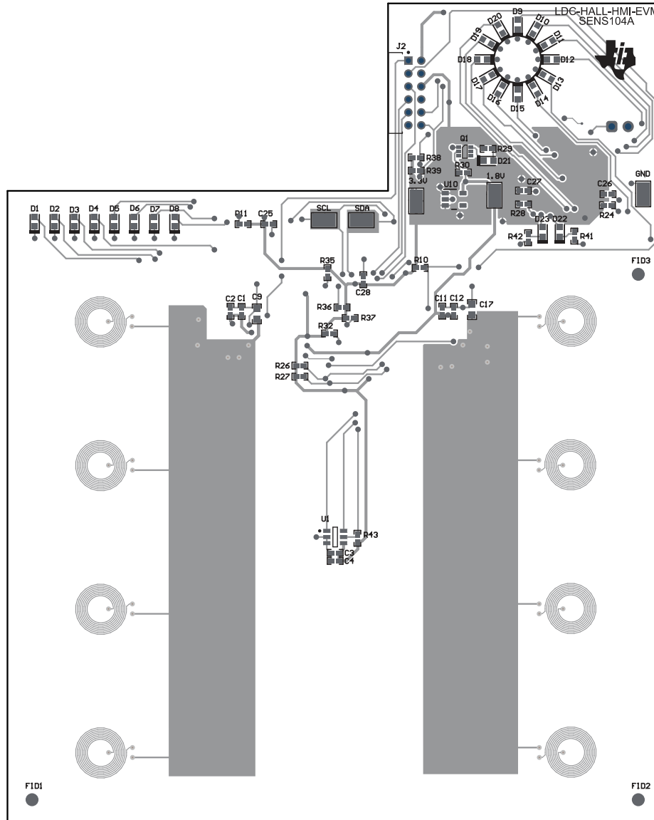
Figure 4-1. Top Layout
