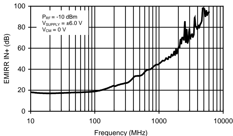
Figure 1. OPA703 EMIRR IN+ vs Frequency
