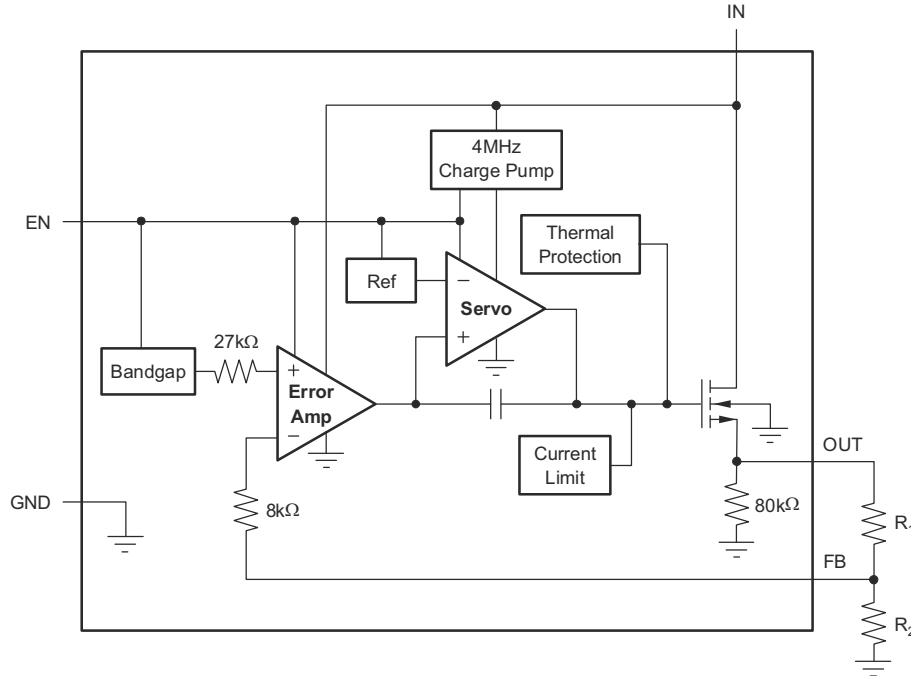
Figure 6-2. Adjustable-Voltage Version
