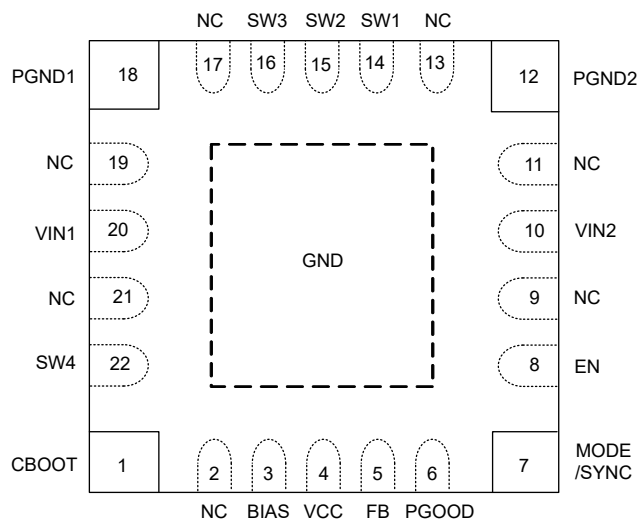
Figure 4-1. Pin Diagram
