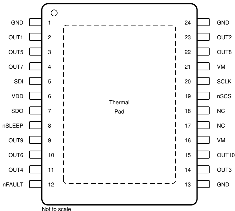
Figure 4-1. Pin Diagram
