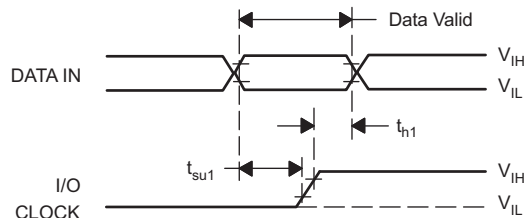
Figure 47. DATA IN and I/O CLOCK Voltage Waveforms
