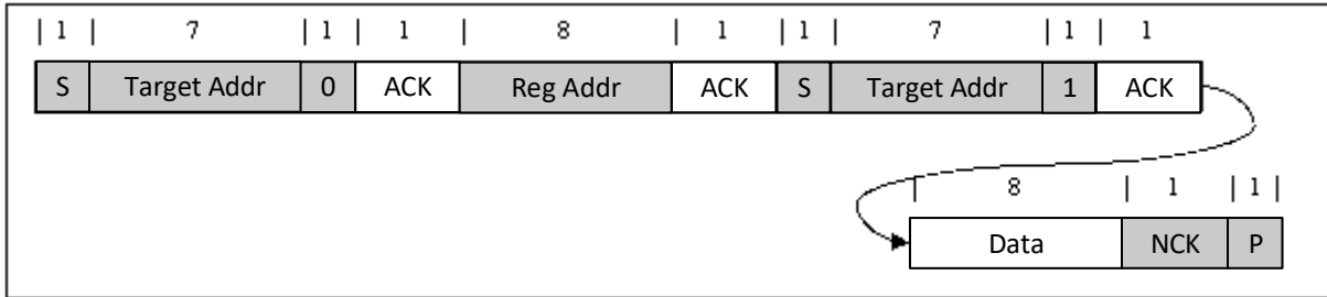
Figure 7-14. Single Read
