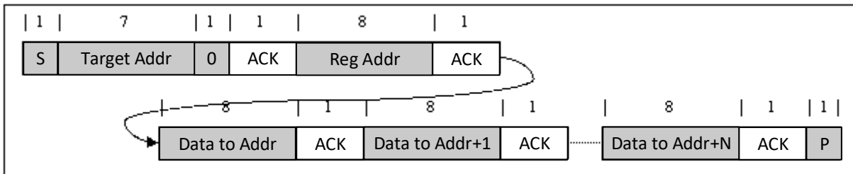
Figure 7-15. Multi-Write
