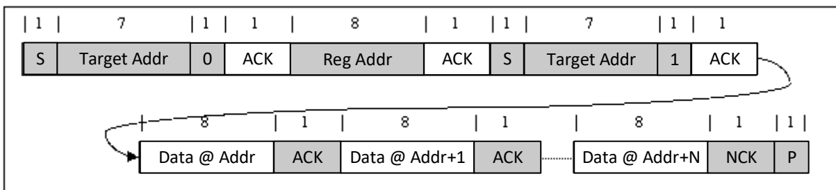
Figure 7-16. Multi-Read
