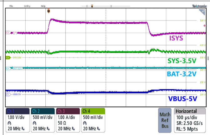
Figure 8-5. Charge Enable
