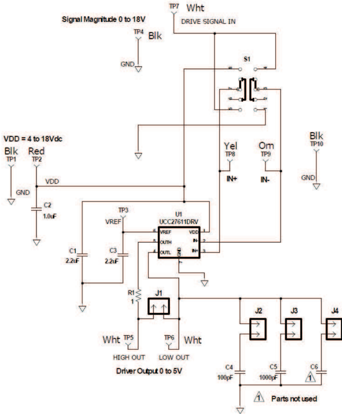
Figure 1. UCC27611OLEVM-203 Schematic
