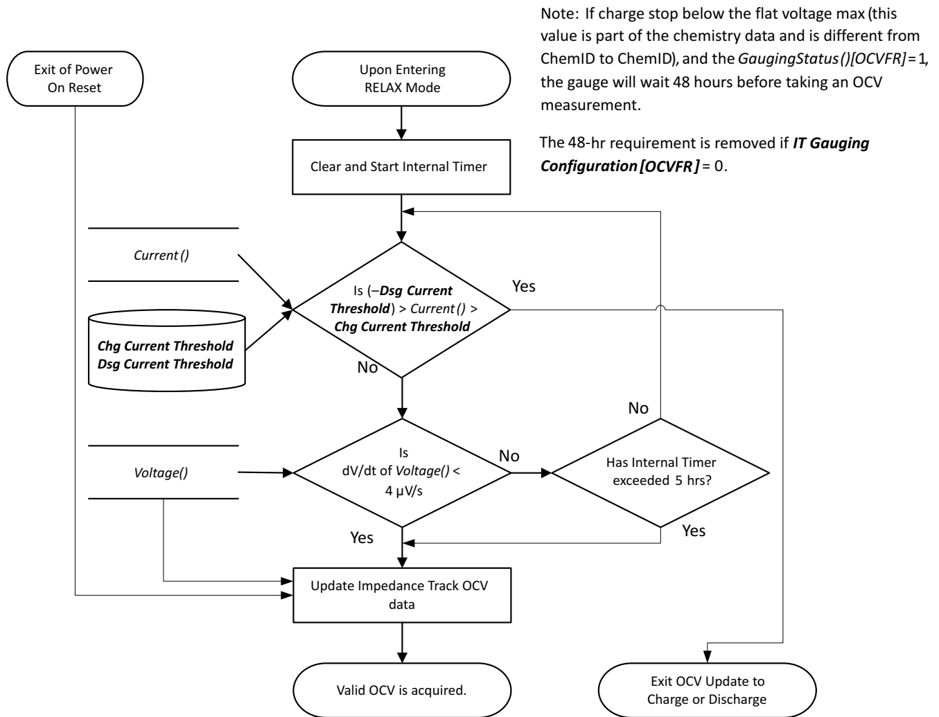
Figure 7-2. OCV Measurement
