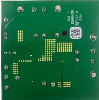
Figure 5-5. TPS563300EVM Board Bottom View
