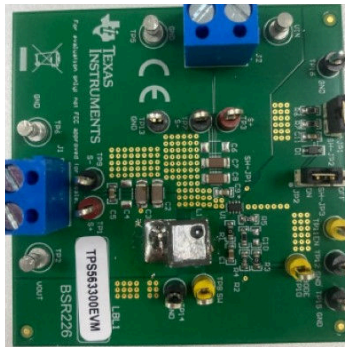
Figure 5-4. TPS563300EVM Board Top View
