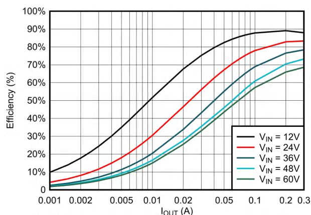
Figure 3-2. Efficiency, V_{OUT} = 5V , 1100kHz(FPWM)
