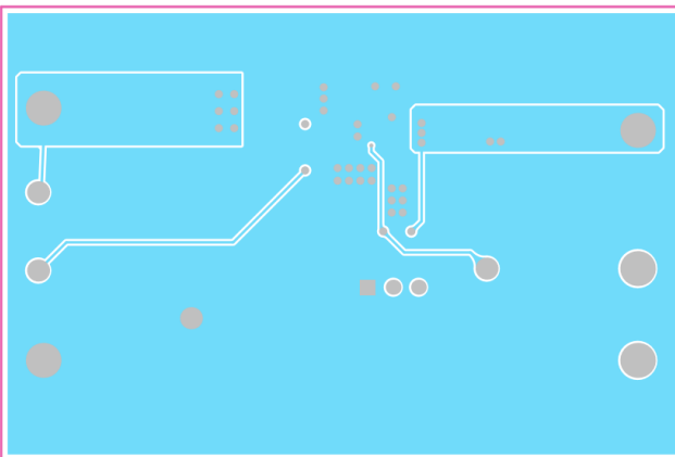
Figure 4-4. Layer 3 Copper (Top View)
