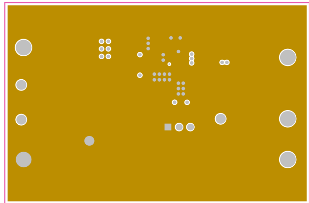
Figure 4-3. Layer 2 Copper (Top View)
