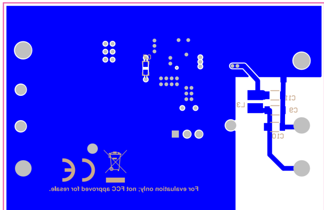
Figure 4-5. Bottom Copper (Top View)
