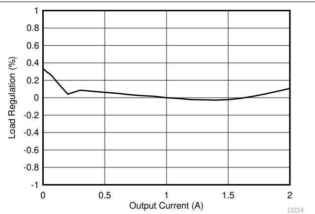
Figure 8-5. TPS562200 Load Regulation, V_I = 12V
