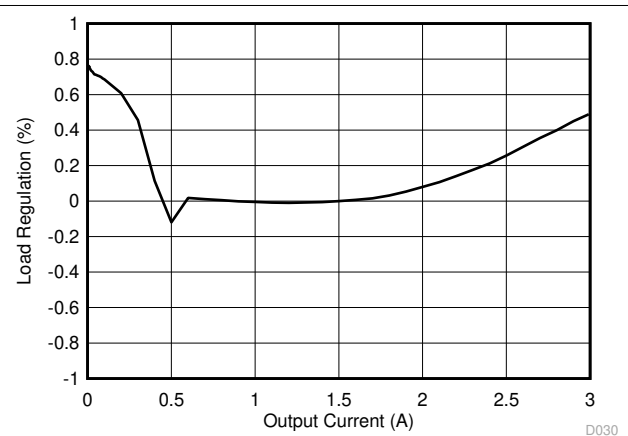
Figure 8-20. Tps563200 Load Regulation, V_I = 12\text{ V}
