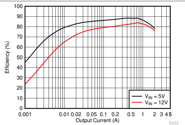
Figure 8-3. TPS562200 Light Load Efficiency
