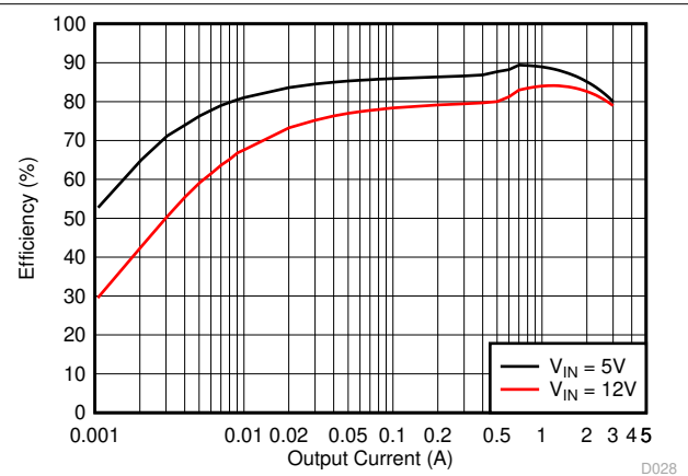
Figure 8-18. Tps563200 Light Load Efficiency
