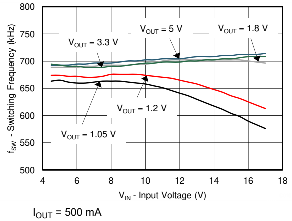
Figure 6-8. Switching Frequency vs Input Voltage I_{OUT} = 500\text{ mA}
