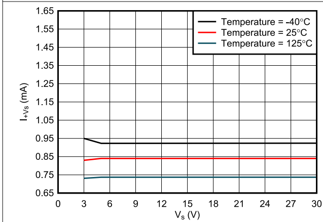
Figure 7-15. I Vs vs Vs in ON State
