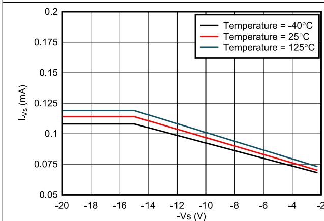
Figure 7-17. I Vs vs -Vs in ON State
