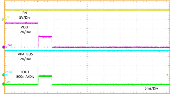
Figure 11-28. OUT short to 5.1- \Omega Load
