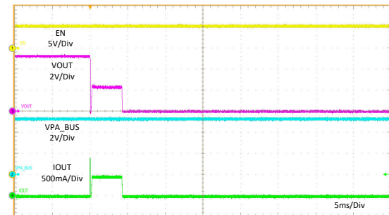
Figure 11-23. 1-Ω Load Recovery
