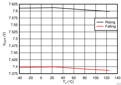
TPS259803x Variants
