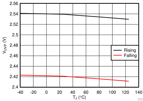
Figure 7-1. Supply UVP Threshold vs Temperature
