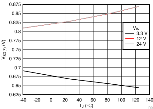
Figure 7-7. EN/UVLO Falling Threshold for Lowest Current Consumption
