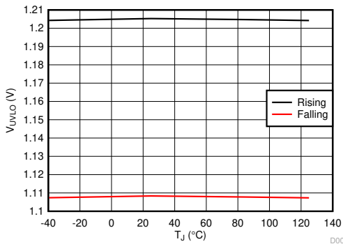
Figure 7-5. EN/UVLO Threshold vs Temperature
