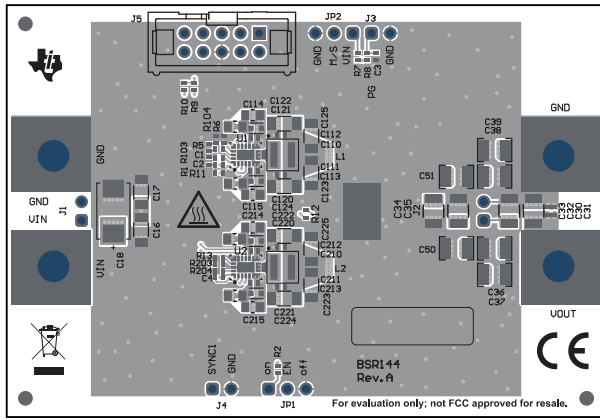
Figure 5-1. Top Layer - Components
