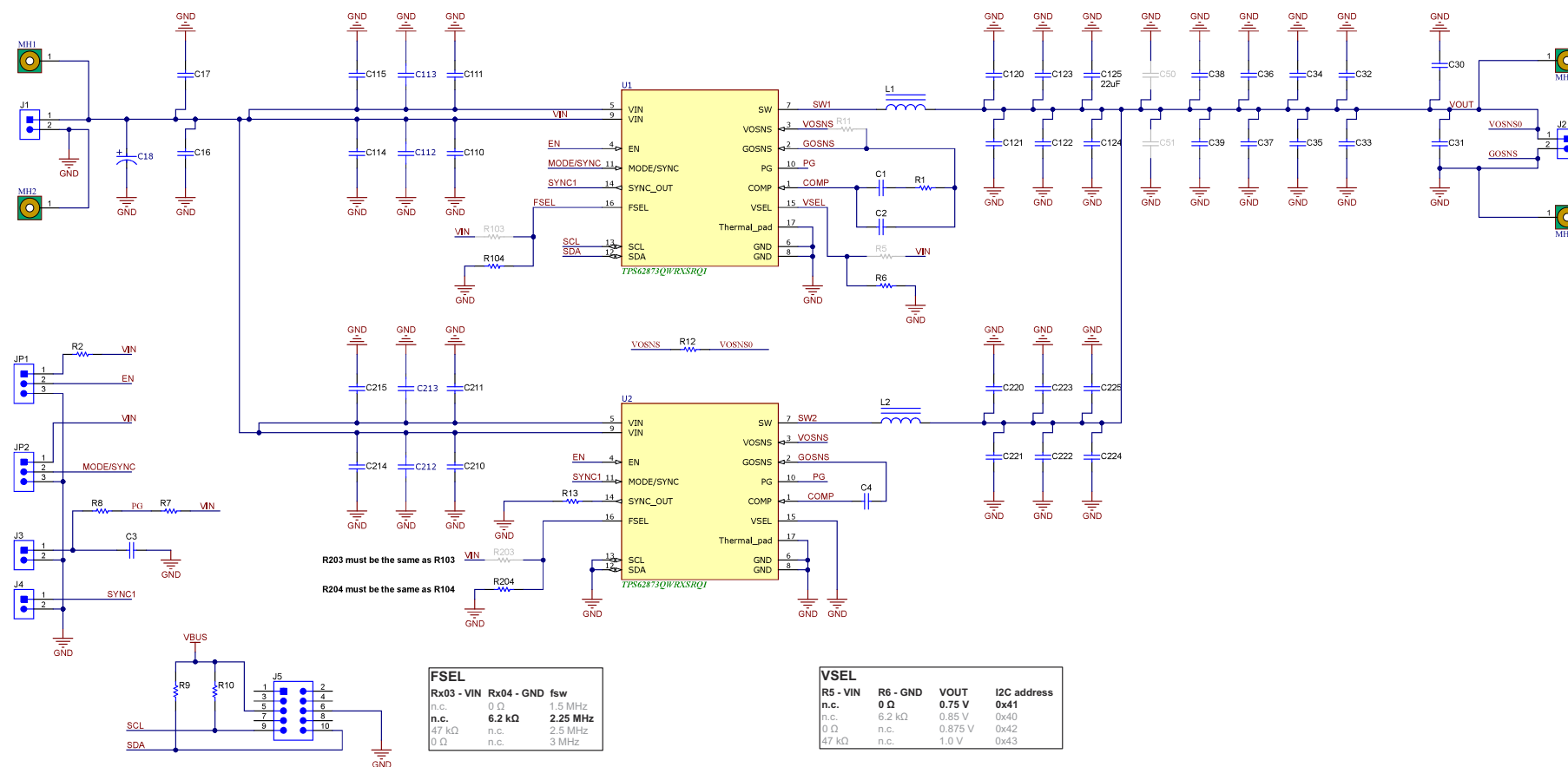
Figure 6-1. TPS62873EVM-144 Schematic
