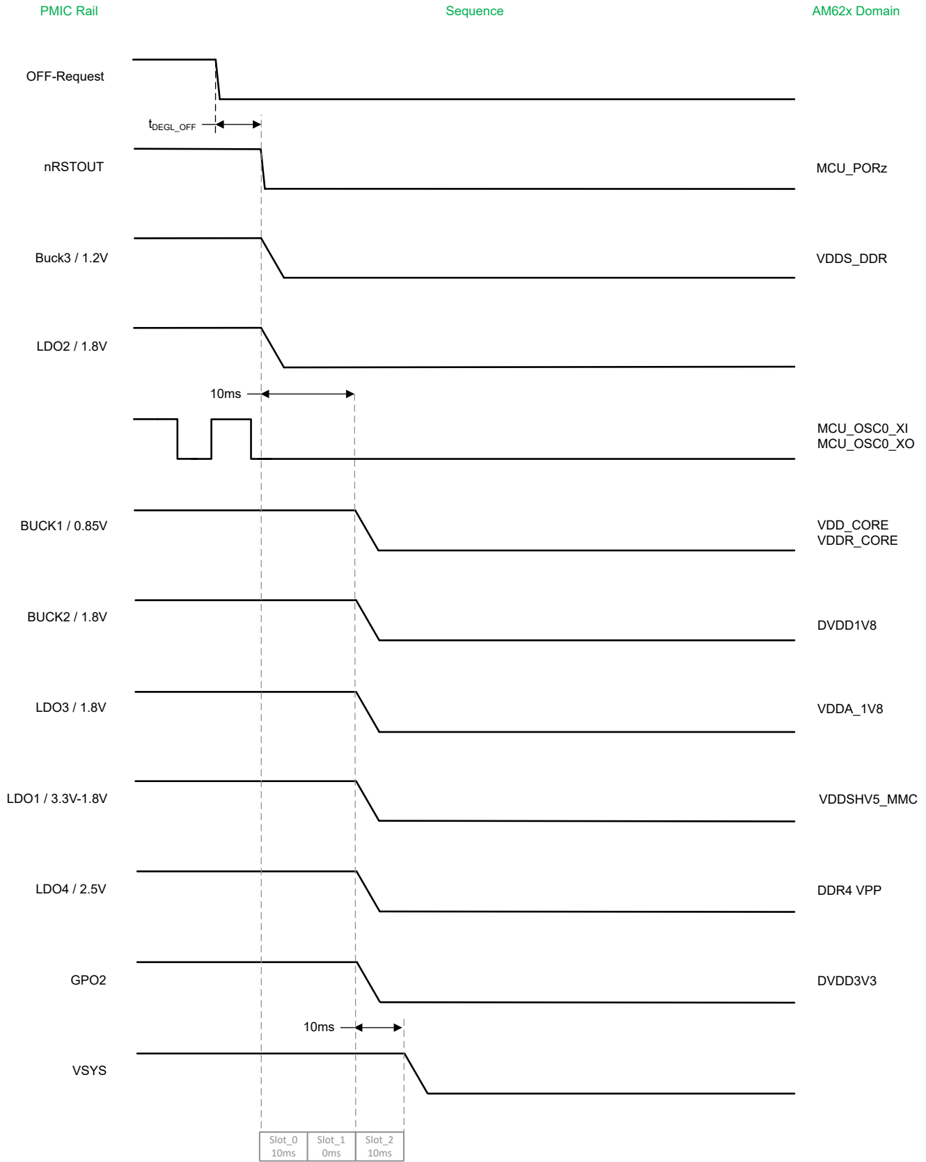
Figure 2-2. TPS6521904 Power-Down Sequence
