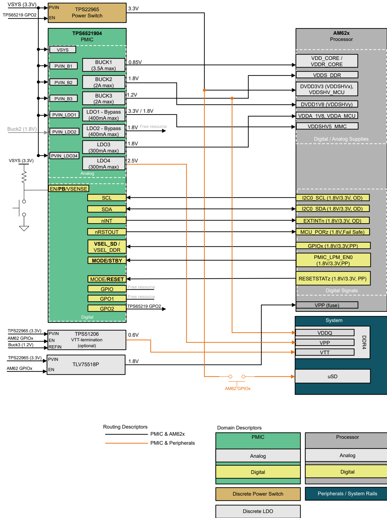
Figure 2-3. TPS6521904 Example Power Block Diagram
