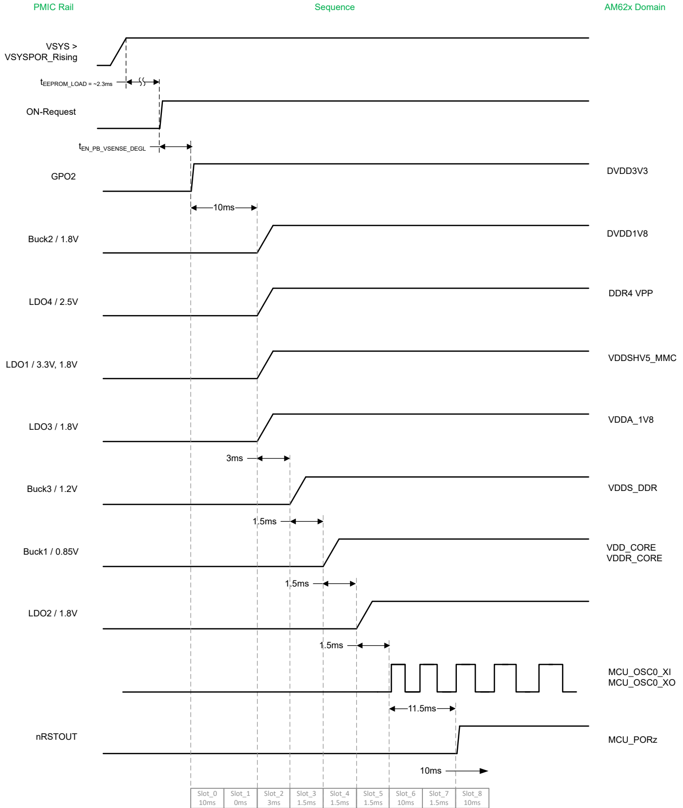
Figure 2-1. TPS6521904 Power-Up Sequence
