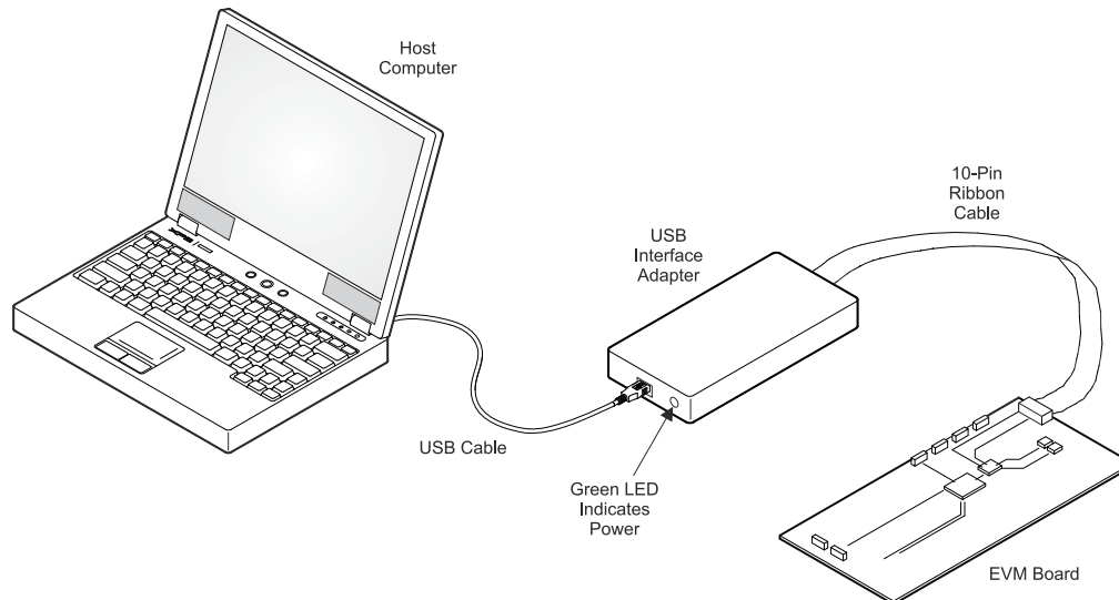
Figure 3-1. Quick Connection Overview
