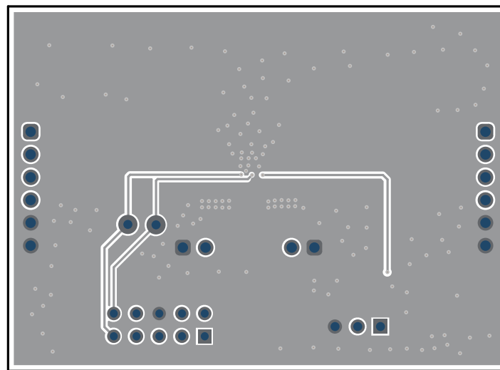
Figure 4-3. TPS631012/3EVM PCB - Bottom Layer (Top View)
