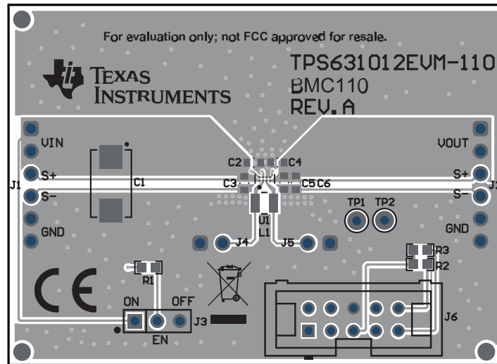
Figure 4-2. TPS631012/3EVM PCB - Top Layer
