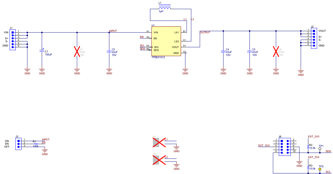
Figure 4-1. TPS631012/3EVM Schematic
