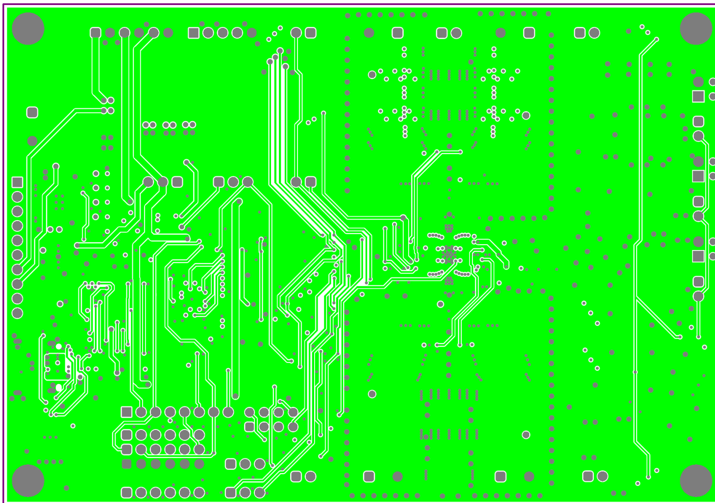
Figure 4-5. Layout Signal, Layer 3
