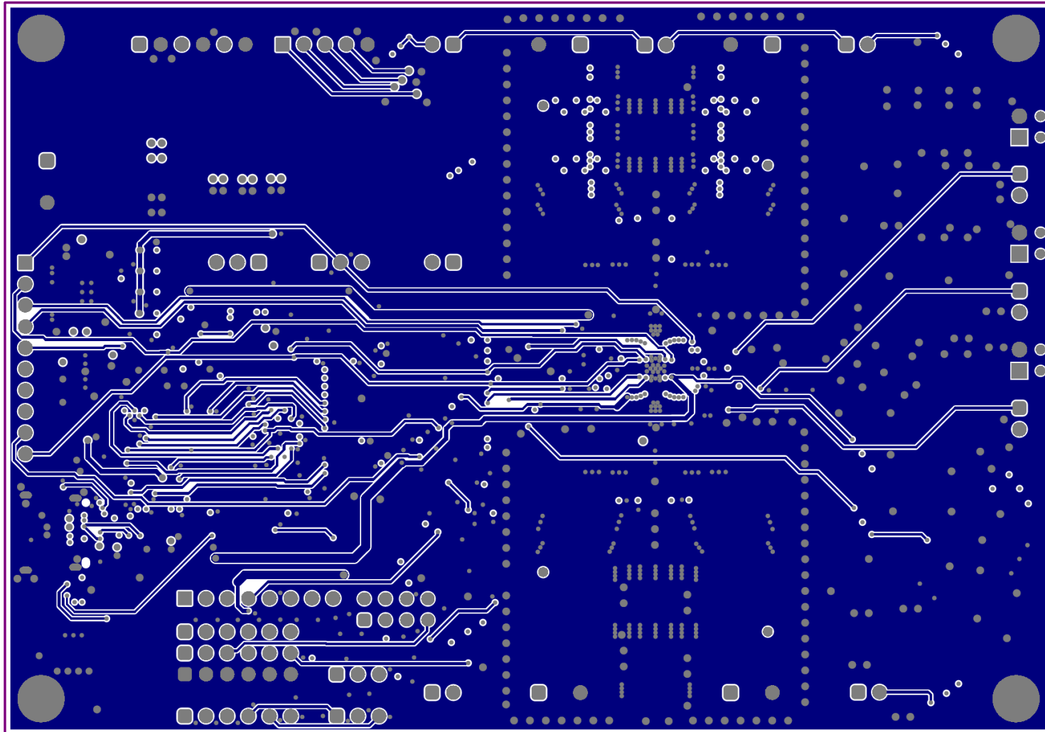
Figure 4-6. Layout Signal, Layer 4
