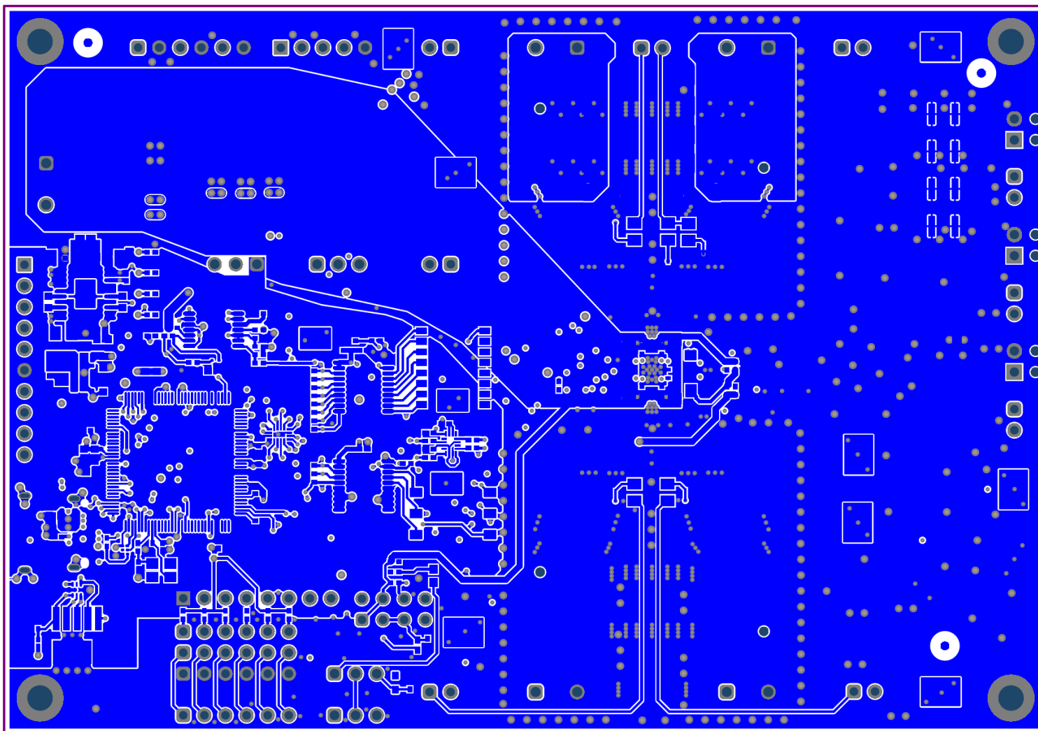
Figure 4-8. Layout Bottom
