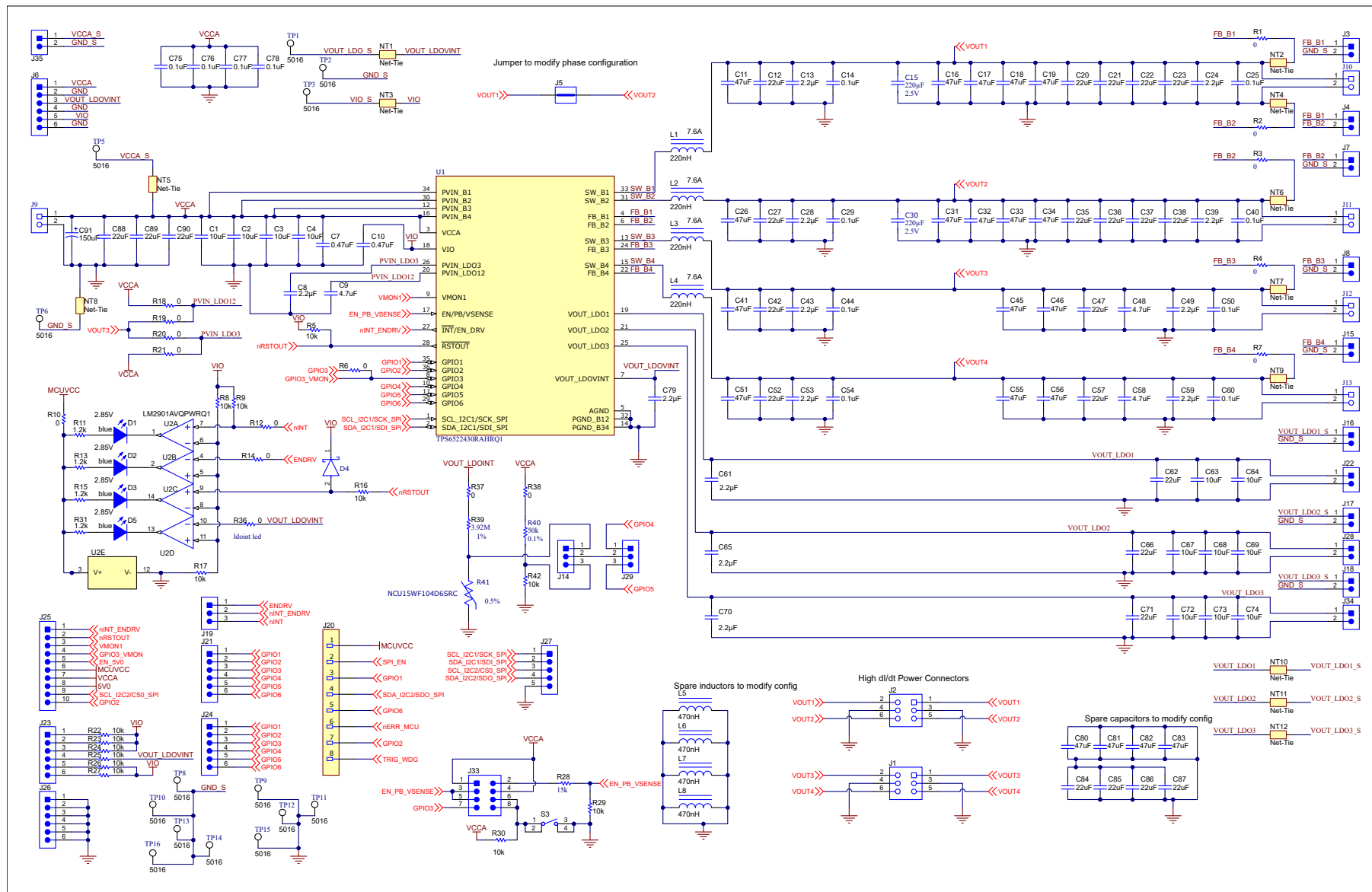
Figure 4-1. Schematic Page 1
