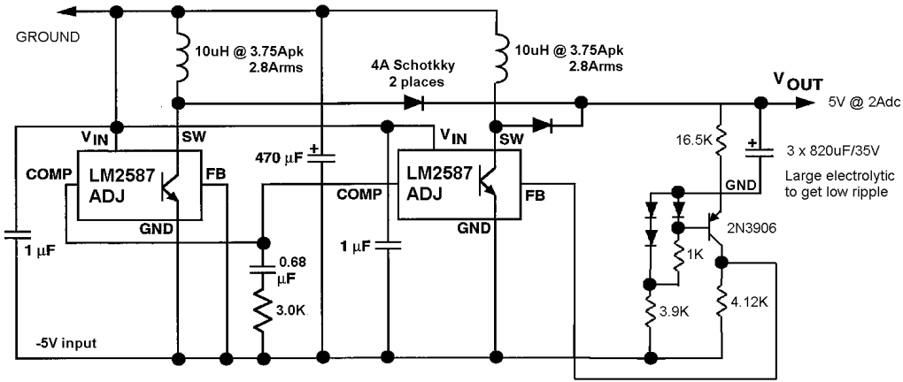
DUAL LM2587 BOOST CIRCUIT
